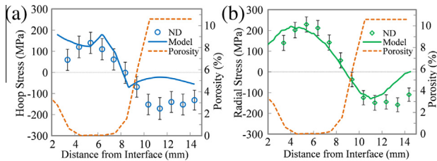
Figure 4. (a) Hoop and (b) radial residual stress distributions in the as-sprayed preform from ND measurements and FE modelling with \mu CT porosity measurements.
