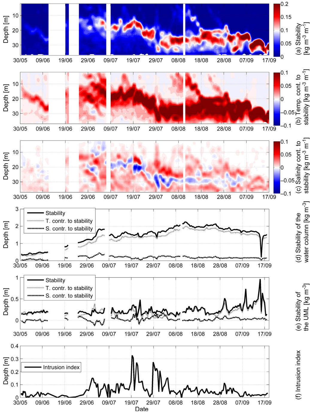
Figure 3 Temporal development of the following vertical stratification parameters at the buoy station from 30 May to 18 September 2015: stability (a; [kg m -3 m -1 ]) and contribution of temperature (b) and salinity (c) to stability; integrated stability parameters [kg m -3 ] for the whole water column (d) and for the upper layer (e); intrusion index (f).
