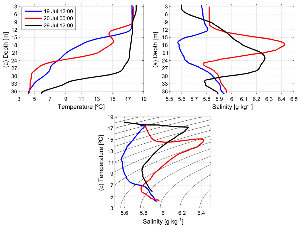
Figure 4 Selected profiles of temperature [ ^{\circ}\text{C} ; a) and salinity [ \text{g kg}^{-1} ; b) and respective temperature–salinity diagram with density anomaly [ \text{kg m}^{-3} ]; c) as contour lines in profiling station (the location is shown as a yellow circle in Fig. 1).
