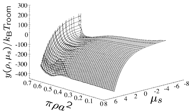
FIGURE 17 Semigrand potential per unit volume y(\rho, \mu_s) as a function of reduced DNA density and salt chemical potential, for the KL model and parameters \theta = 0.9, f_1 = 0.3, f_2 = 0.7, and f_3 = 0 .
