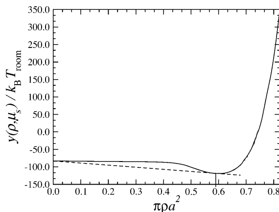
FIGURE 18 Semigrand potential per unit volume y(\rho, \mu_s) on a line of constant DNA chemical potential for the KL model as a function of the reduced DNA density and for parameters \theta = 0.9, f_1 = 0.3, f_2 = 0.7, and f_3 = 0 . Also shown (dashed line) is the common tangent connecting the coexisting phase points.
