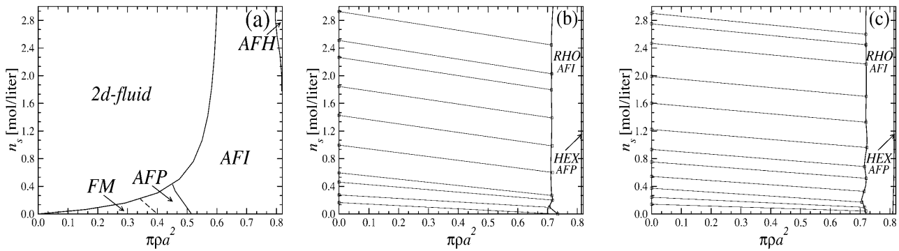
FIGURE 14 Phase diagrams of DNA-salt mixtures for the YS model as a function of the DNA packing fraction \pi\rho a^2 and salt concentration n_s in the aggregate: (a) \theta = 0.9, f_3 = 1 ; the lattice here is HEX . (b) \theta = 0.7, f_1 = 0.3 , and f_2 = 0.7 ; (c) \theta = 0.9, f_1 = 0.3 , and f_2 = 0.7 . Dashed lines denote second-order magnetic transitions, solid lines first-order ones. The geometrical transitions between different lattices in b and c are second order; the straight lines are tielines between coexisting phases.
