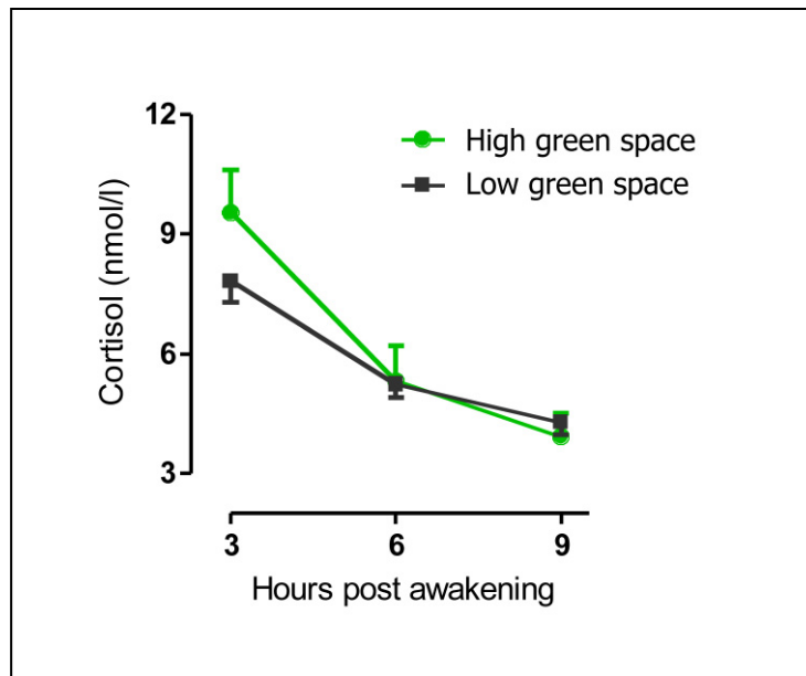
Fig 2. Difference in cortisol slope between participants living in high versus low greenspace areas (First published in Roe et al., 2013).
