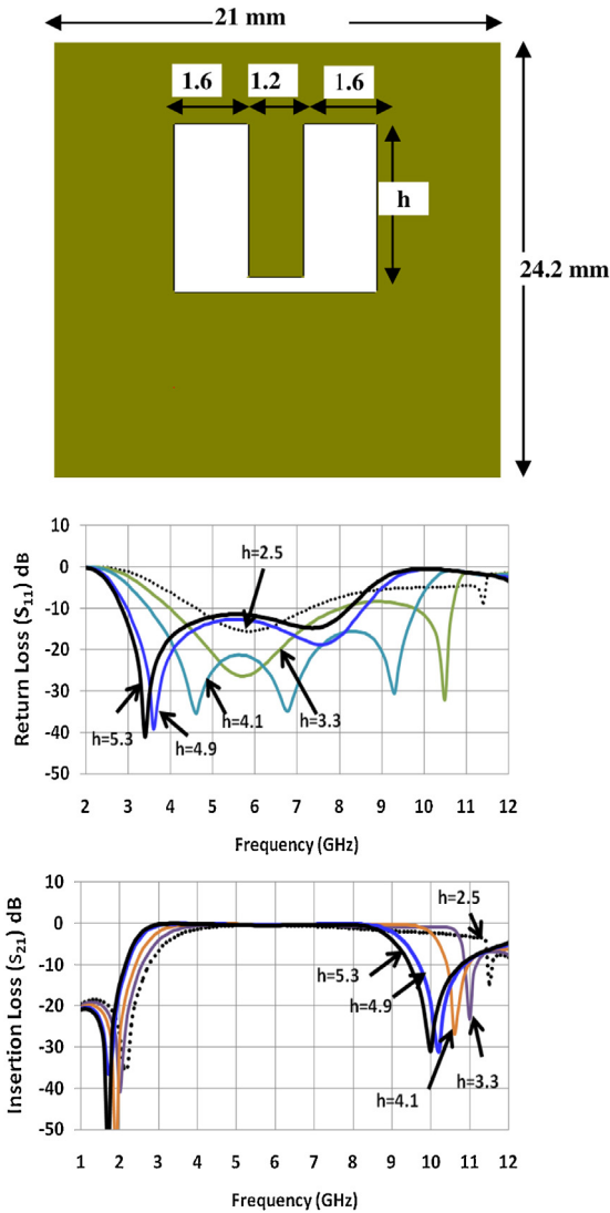
Fig. 5. The filter performance against different U-slot height ( h ).
