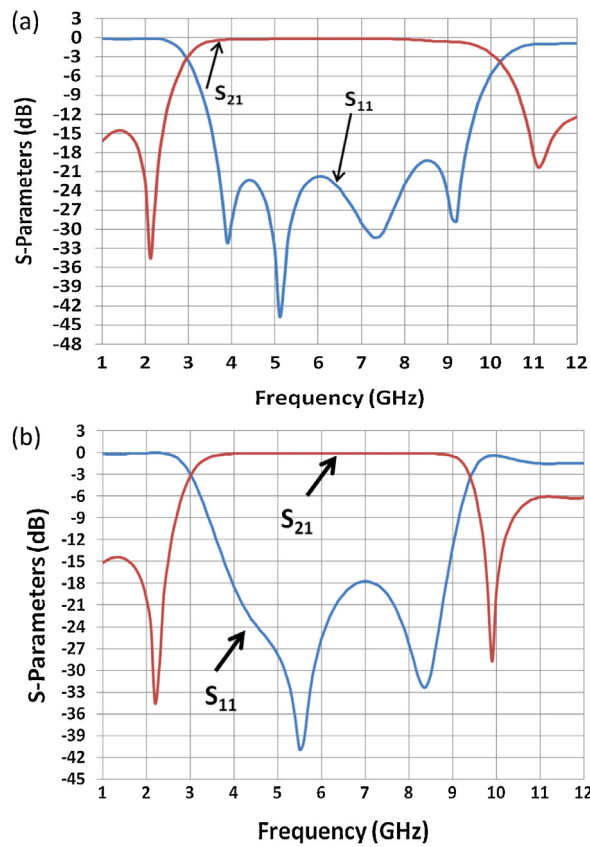
Fig. 7. The S-parameter simulation results for the proposed UWB-BPF. (a) IE3D simulation. (b) HFSS simulation.
