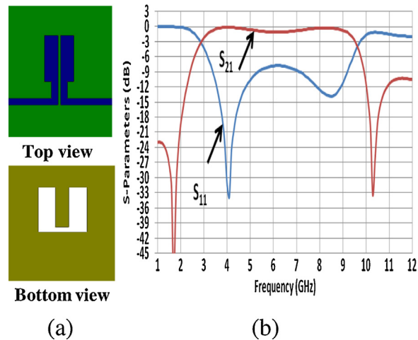
Fig. 1. (a) UWB-BPF with regular coupled lines and U-slot DGS. (b) Simulation results.
