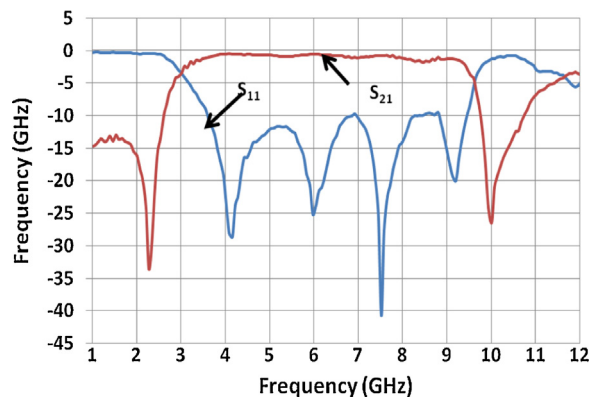
Fig. 10. The measured S -parameters for the realized UWB-BPF.
