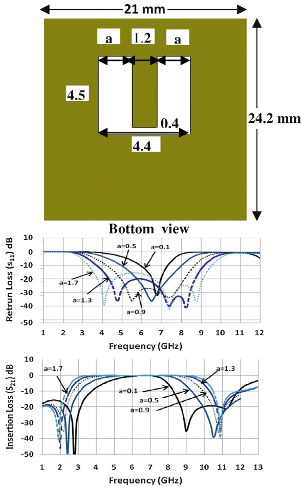
Fig. 3. The filter performance against different U-slot widths ( a ).
