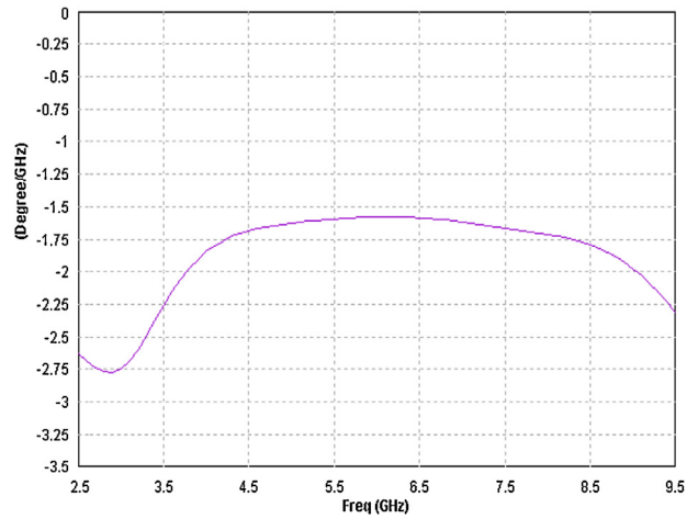
Fig. 8. The simulated group delay of the proposed bandpass filter.
