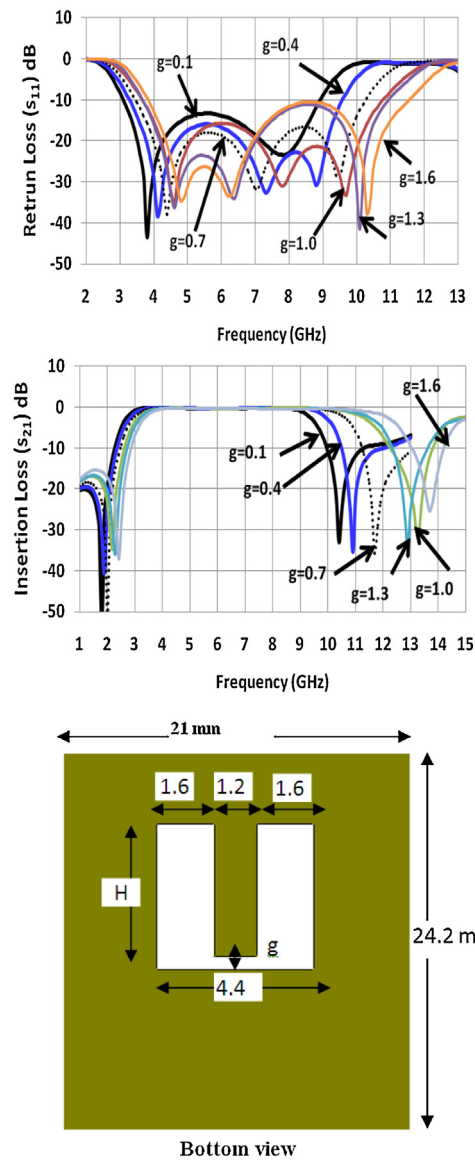
Fig. 4. The filter S-parameters against frequencies for different U-slot gap ( g ).
