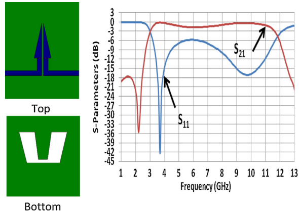
Fig. 2. UWB-BPF simulation for arrow coupled lines and reshaped U-slot DGS.
