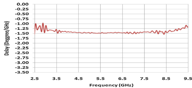
Fig. 11. The measured group delay for the realized UWB-BPF.
