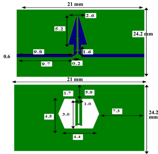
Fig. 6. The UWB-BPF dimension for upper and lower side.
