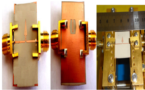
Fig. 9. The photos of the realized UWB-BPF.
