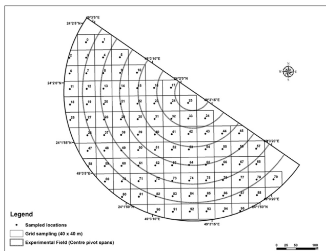
Figure 2 Grid sampling map of the experimental field.
