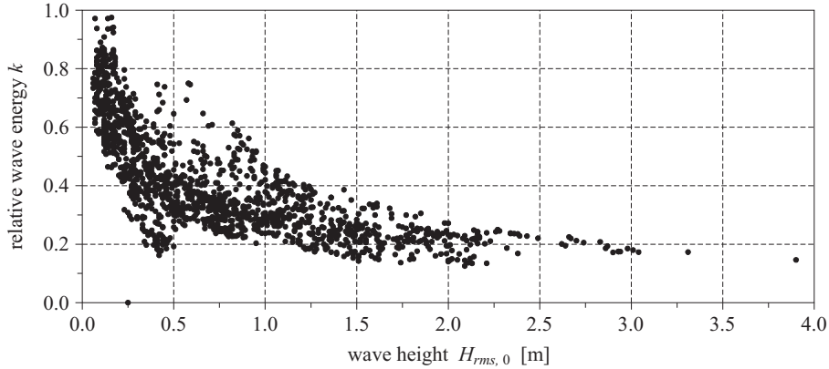
Figure 6. Variability in relative nearshore wave energy k at depth h \approx 0.5 m with respect to deep-water energy (at h = 15 m) for root-mean-square offshore wave heights H_{rms,0} \in (0.06; 3.9) m
