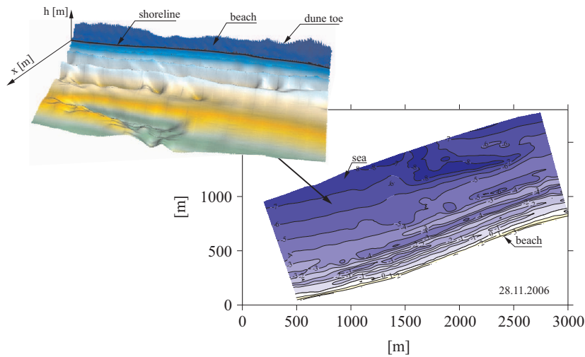
Figure 3. Spatial configuration of the coastal section at Lubiatowo
