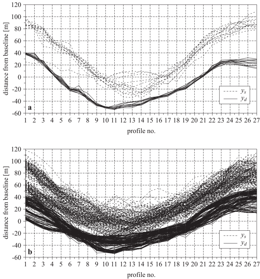
Figure 4. Shoreline and dune toe positions y_s and y_d in the period from September 2006 to September 2007 (a) and in the period from 1983 to 2007 (b)
