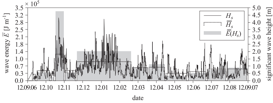
Figure 8. Hourly \overline{H}_s and time-averaged ( \overline{H}_s ) significant wave heights together with wave energy \overline{E} averaged over time periods \Delta t_k
