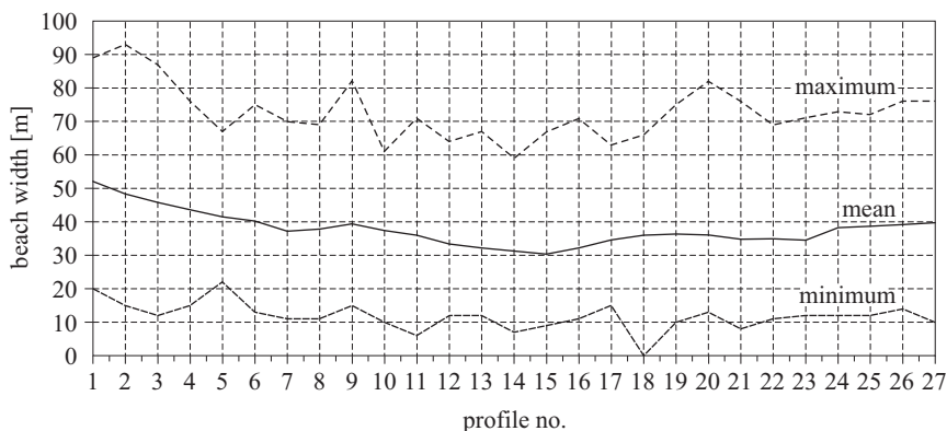
Figure 7. Mean beach width and its minimum and maximum envelope for 27 profile lines
