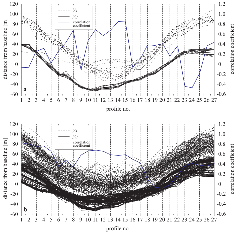
Figure 11. Variability in shoreline and dune toe locations at CRS Lubiatowo in the year from September 2006 to September 2007 (a) and in the long-term period from 1983 to 2007 (b)
