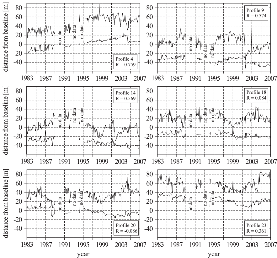
Figure 10. Variability in shoreline and dune toe locations for selected cross-shore profiles at CRS Lubiatowo in 1983–2007
