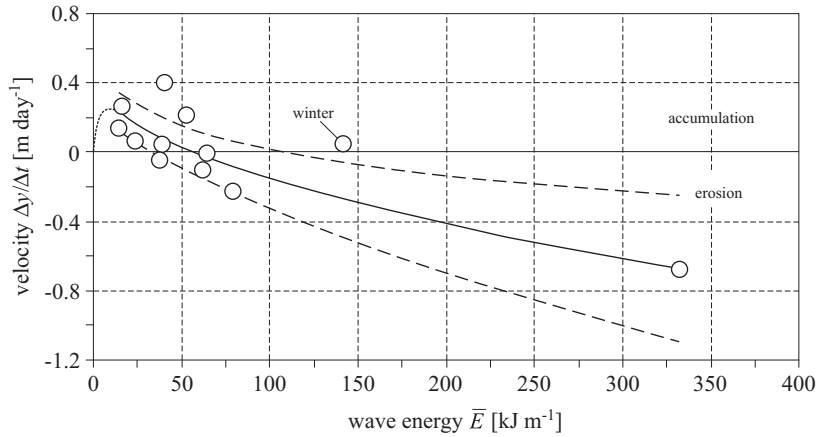
Figure 9. Velocity of shoreline migration as function of wave energy \overline{E} \in (14; 333) \text{ kJ m}^{-1}
