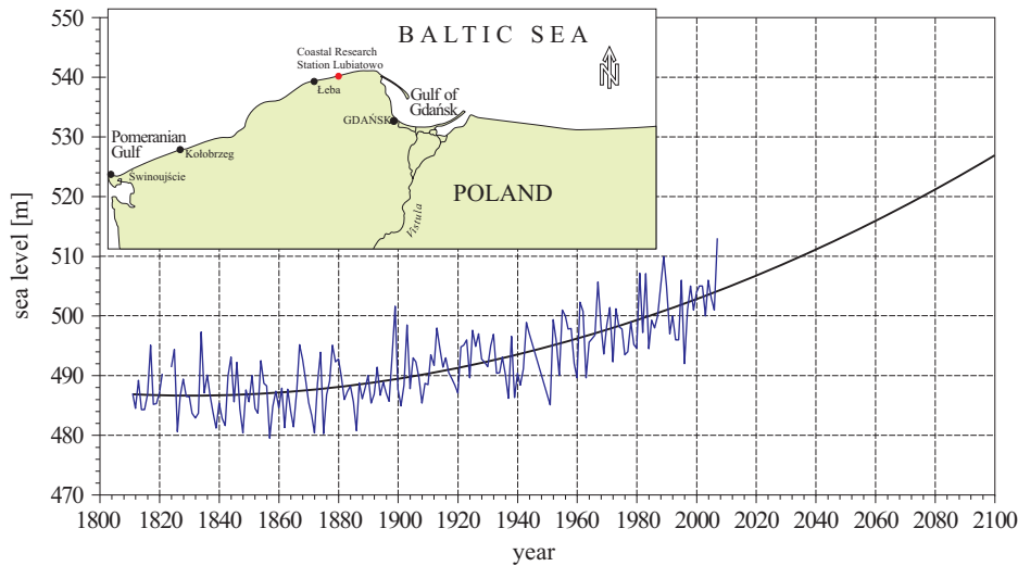
Figure 1. Increasing trend of sea level rise detected in long-term data registered at the southern Baltic measuring station at Świnoujście (Poland)
