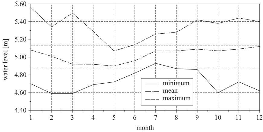
Figure 5. Monthly mean and mean monthly extreme sea levels at the Łeba gauge in 1951–2000; data after Girjatowicz (2009)
