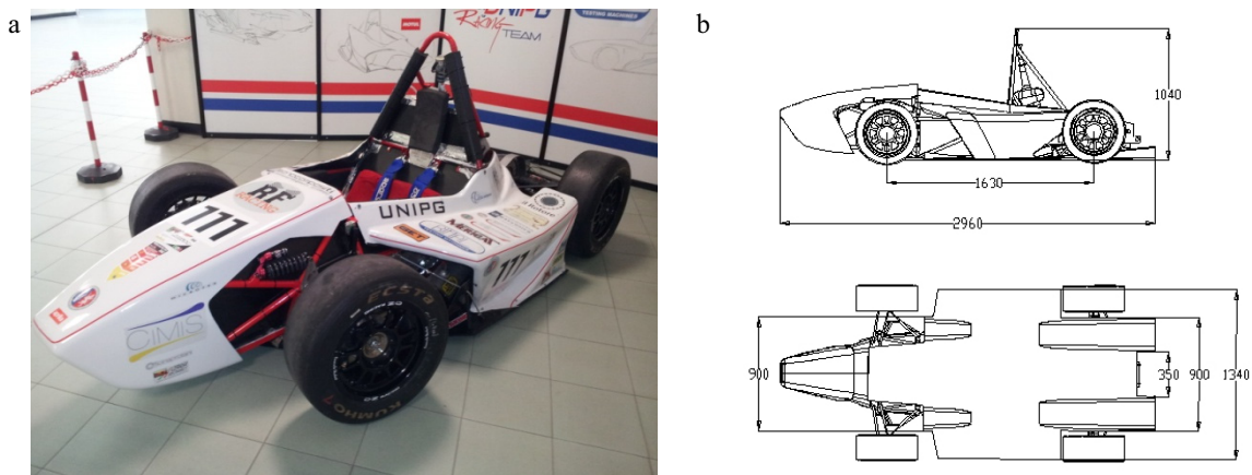
Fig. 1. (a) Formula SAE racing car; (b) Characteristics measures of the car (all dimensions are in mm).
