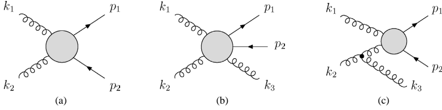
Fig. 1. Generic structure of (a) LO diagrams, (b) NLO real correction diagrams, (c) NLO diagrams giving rise to a collinear divergence for k_3 \rightarrow (1-x)k_2 .
