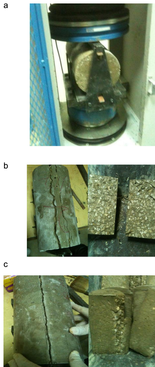
Fig. 6. (a) Splitting tensile strength device, (b) failure of monolithic cylinder, (c) failure of a non-monolithic (CJ) cylinder.
