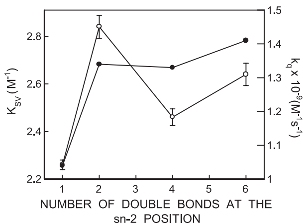
Fig. 6. Stern–Volmer quenching constants, K_{SV} (O) and bimolecular quenching constants, k_q (●) for acrylamide quenching of melittin bound to membranes of varying degrees of unsaturation. The bimolecular quenching constants were calculated using Eq. (5). The excitation wavelength was 295 nm and emission was monitored at 337 nm. The data points shown are the means \pm S.E. of three independent measurements. The ratio of melittin to lipid was 1:50 (mol/mol) and the concentration of melittin was 3.2 \mu M in all cases. See Materials and methods for other details.
