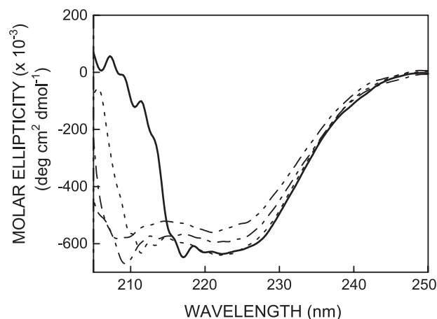
Fig. 7. Effect of increasing number of double bonds at the sn-2 fatty acyl chain on the far-UV CD spectra of melittin bound to membranes composed of varying degrees of unsaturation corresponding to POPC (---), PLPC (-.-.), PAPC (---), and PDPC (—). The ratio of melittin to lipid was 1:50 (mol/mol) and the concentration of melittin was 17.0 \mu M in all cases. See Materials and methods for other details.
