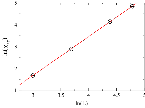
Fig. 2. Log–log plot plot of the maxima of the planar susceptibility as a function of the lattice size. The solid line shows the best linear fit of the data given the exponent \gamma/\nu=1.763(1) . The error bars are shown inside the symbols.
