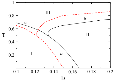
Fig. 1. Phase diagram of the anisotropic Heisenberg model with dipolar interactions (AHd) for fixed A/J = 1 in the (D/J, T) space. The solid (black) line represents the transition lines as obtained using a cut-off in the dipolar interactions [12] and the dashed (red) line is the results obtained when full long-range interactions are considered by means of the Ewald summation (this work). The phase I is an Ising-like phase characterized by an ordered out-of-plane alignment of spins (that may present stripe-like configurations for full long-rang interactions). Phase II is an ordered planar ferromagnetic state and phase III is a paramagnetic one. The border line between phase I and phase II ( a ) is believed to be of first order and from regions I and II to III ( b and c ) to be both of second order.
