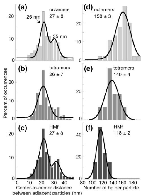
Figure 3. Quantitation of Center-to-Center Distances between Adjacent Particles and Number of Base Pairs per Particle from Fibers in AFM Images
