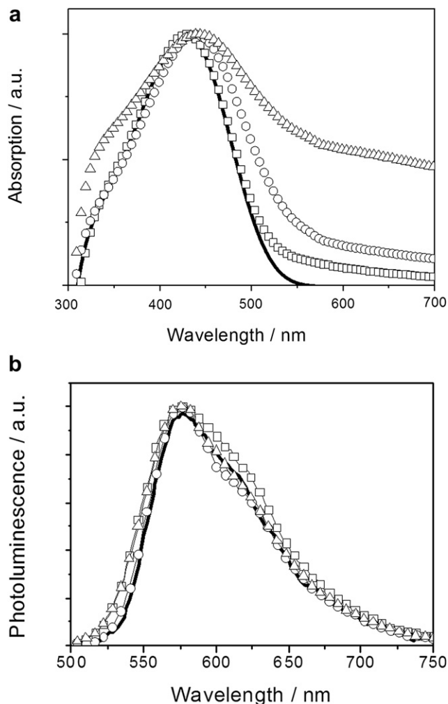
Fig. 1. Normalized (a) absorption and (b) photoluminescence spectra of 1 mg mL -1 chloroform solution of (●) P3HT, (□) P3HT-Au, (○) P3HT-C 60 and (△) P3HT-C 60 -Au.
