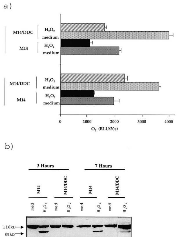
Fig. 3. Inhibition of intracellular Cu/Zn SOD retards H 2 O 2 -induced decrease in intracellular O 2 - concentration and caspase activity. a: Intracellular O 2 - concentration in M14 and M14/DDC cells (1 mM DDC) was evaluated following 3 and 7 h incubation of 2 × 10 6 cells with serum-free DME alone (medium) or supplemented with 0.5 mM H 2 O 2 (H 2 O 2 ). Intracellular O 2 - concentration was assessed as in Fig. 2. b: Western blot analysis of PARP cleavage following 3 and 7 h incubations of M14 and M14/DDC cells in serum-free medium alone (med) or supplemented with 0.5 mM H 2 O 2 (H 2 O 2 ). Western blot analysis was performed as described in Fig. 1.
