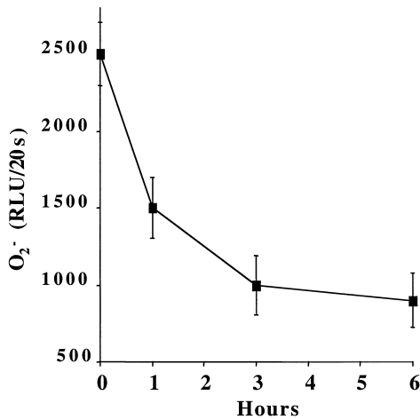
Fig. 2. H 2 O 2 -mediated apoptosis is associated with a decrease in the intracellular O 2 - concentration. Intracellular O 2 - concentration of M14 cells (2 × 10 6 ) was assessed following incubation with 0.5 mM H 2 O 2 for 1, 3, and 6 h. Level of intracellular O 2 - was measured by a lucigenin-based chemiluminescence assay. Data are shown in relative light units per 20 s (RLU/20s) ± S.E.M from two independent measurements.
