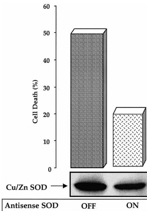
Fig. 5. Decrease in intracellular Cu/Zn SOD protein inhibits H_2O_2 -induced apoptosis. Western blot analysis of Cu/Zn SOD expression in lysates of M14 AS-SOD3 clone ( 5 \times 10^6 cells) cultured in the presence of 2 \mu\text{g}/\text{ml} of tetracycline (OFF) or 48 h after the removal of tetracycline (ON). 30 \mu\text{g} of total protein was subjected to 10% PAGE, transferred to nitrocellulose, blotted with 2 \mu\text{g}/\text{ml} of a polyclonal sheep anti-human Cu/Zn SOD for 1 h at room temperature. The Cu/Zn SOD protein was detected using a 1:5000 dilution of an anti-sheep HRP-conjugated IgG and visualized by the Super Signal Substrate Western Blotting Kit. Determination of the percentage cell death was performed using crystal violet staining after 18 h incubation of M14 cells in presence of 0.5 mM H_2O_2 .
