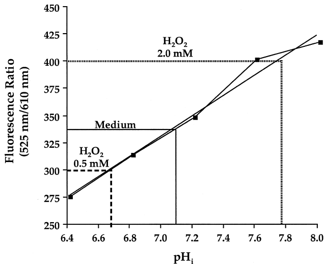
Fig. 7. Apoptotic concentration of H 2 O 2 induces intracellular acidification. M14 cells ( 2 \times 10^6 ) were incubated for 2 h in serum-free DME (medium) or serum-free DME containing 2.0 mM or 0.5 mM H 2 O 2 before intracellular pH was measured by obtaining the fluorescence ratio (525/610 nm) of cells loaded with BCECF, and plotted against a standard curve generated by nigericin (20 \mu M) treatment of cells loaded with BCECF in a high K + buffer at various pH values (6.4–8.0), as described in Section 2.
