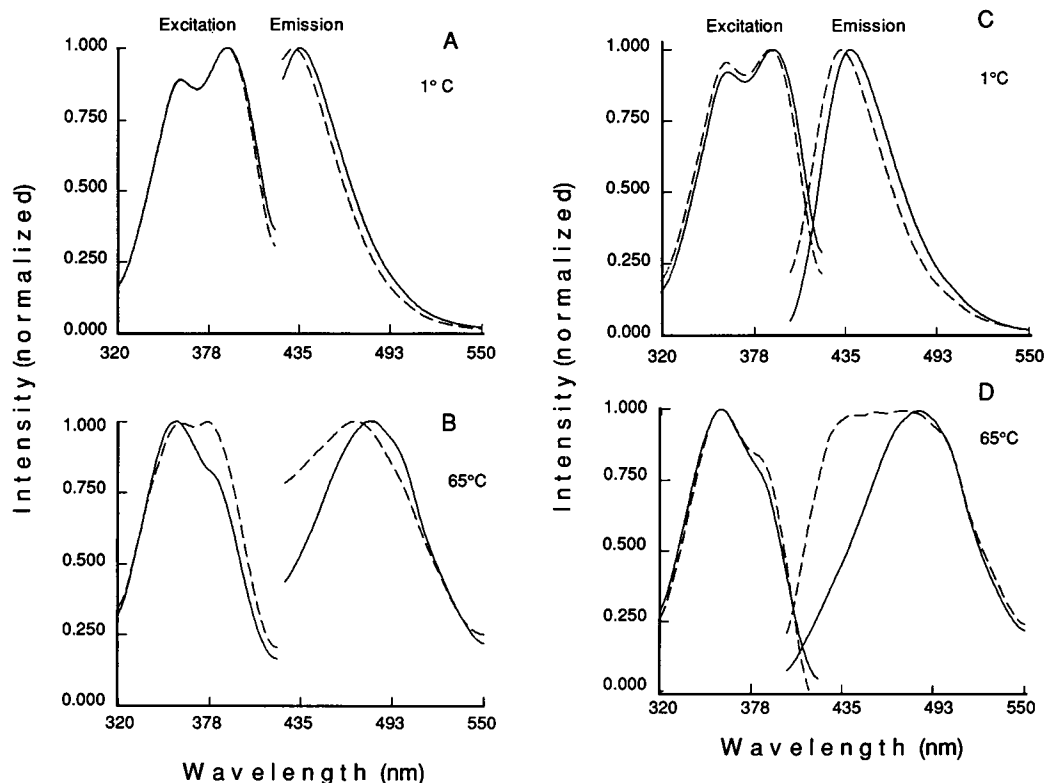
FIGURE 1 Laurdan normalized excitation and emission spectra obtained in multilamellar vesicles composed of DMPC (A and B) and of an equimolar DLPC-DPPC mixture (C and D) with no cholesterol (—) and with 30 mol % cholesterol (---) at 1°C (A and C) and at 65°C (B and D).
