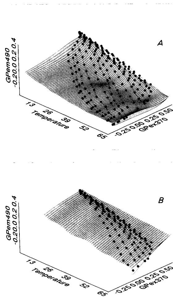
FIGURE 11 Three-dimensional surface obtained as reported in Fig. 9 from Laurdan excitation and emission GP values and from the temperature of their measurement in vesicles composed of DLPC with cholesterol concentrations of (A): 0, 3, 5, 10, 15, 20, 25, 30, 35, 40, 45, and 50 mol %; (B): 25, 30, 35, 40, 45, 50, 55, and 60 mol %. The excitation GP values were measured using excitation at 370 nm and the emission GP values using emission at 490 nm. In both figures the individual three-dimensional curves of samples at each cholesterol concentration are superimposed.
