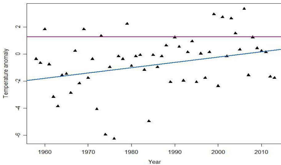
Fig. 1. Tibooburra January maximum temperature anomaly (°C). The horizontal red line is +1.32°C temperature anomaly representing the 90% threshold used to classify the months with extreme heat (those months identified above the red line). The blue line represents the linear fit.
