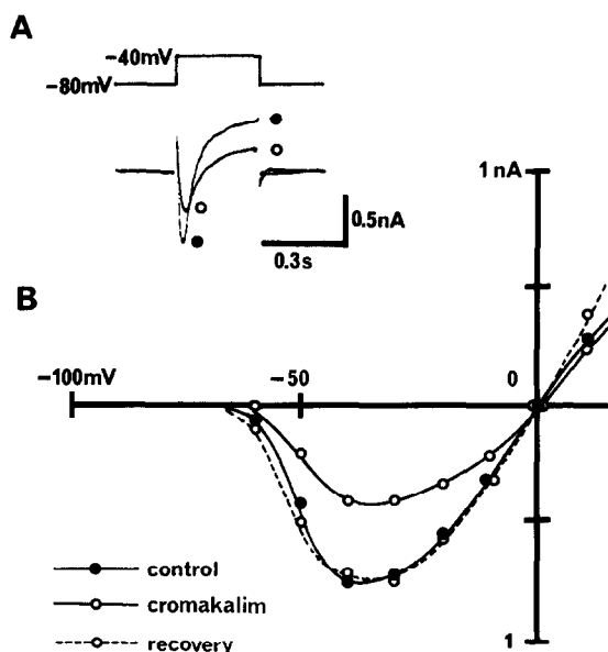
Fig.1. Effects of cromakalim on low-threshold transient calcium currents of NG108-15 cells. A. Ca 2+ inward currents elicited in one cell, by going from a holding potential of -80 mV to a test potential of -40 mV before (●) and during (○) application of 500 μM cromakalim. B. Current-voltage plot of Ca 2+ currents at peak before, during, and after cromakalim, as indicated.
