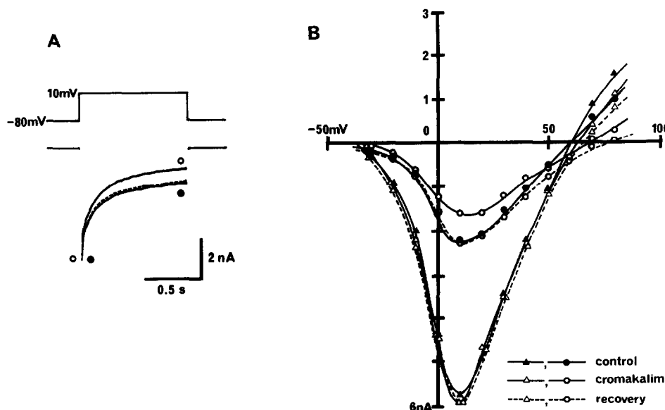
Fig.2. Effect of cromakalim on high-threshold Ba 2+ currents of NG108-15 cells. A. The traces show Ba 2+ currents recorded during 1 s steps from a holding potential of -80 mV to a command potential of +10 mV in the presence (○) and absence (●) of 500 μM cromakalim. Note that no decrease at the peak current (the N-component) but reduction of the long-lasting current (the L-component) at the end of the command pulse was observed. B. Current-potential plot of Ba 2+ currents at peak (Δ, ▲) and after 1 s (○, ●) and during (Δ, ○) cromakalim application, as indicated.
