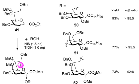
Scheme 10. Activation of benzyl glycal ester with NIS/TfOH.
