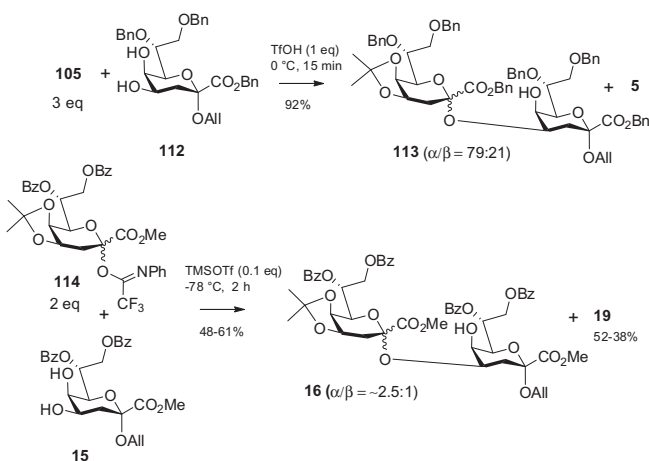
Scheme 19. Kdo disaccharide synthesis with Kdo N -phenyl trifluoroacetimidates.
