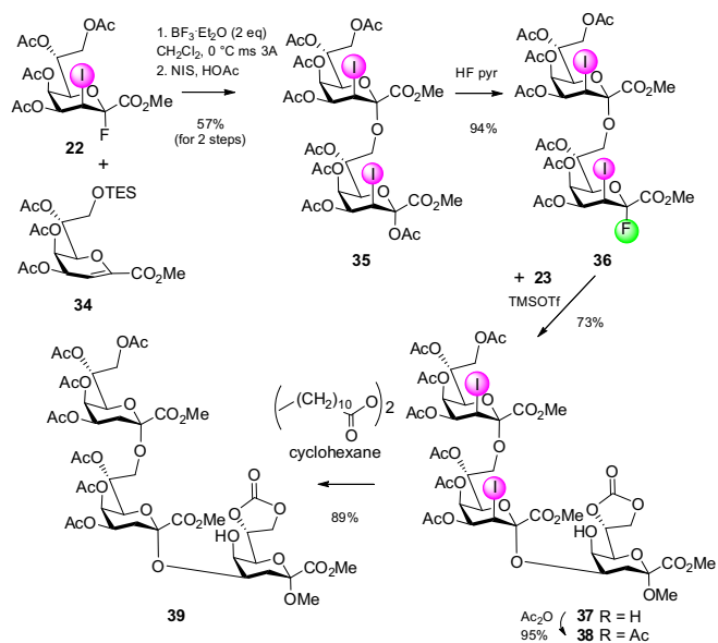
Scheme 7. Synthesis of the linear Chlamydia-specific Kdo trisaccharide 39.
