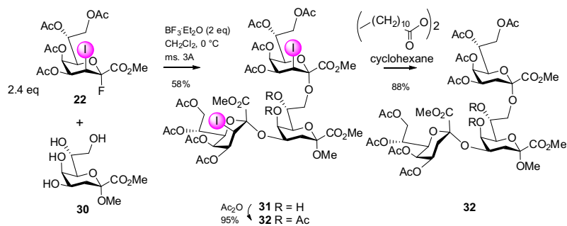
Scheme 6. Synthesis of a 4,8-dibranched Kdo trisaccharide.
