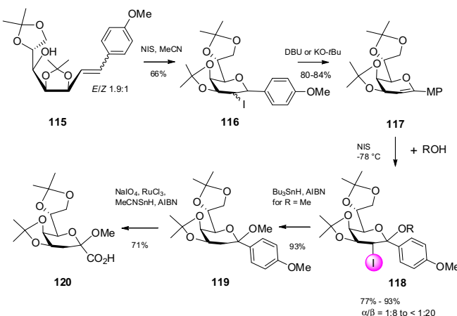
Scheme 20. β-Kdo synthesis from 1-C-aryl glycol.
