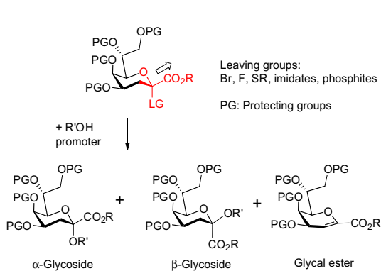
Figure 2. Glycosylation products of Kdo donors.
