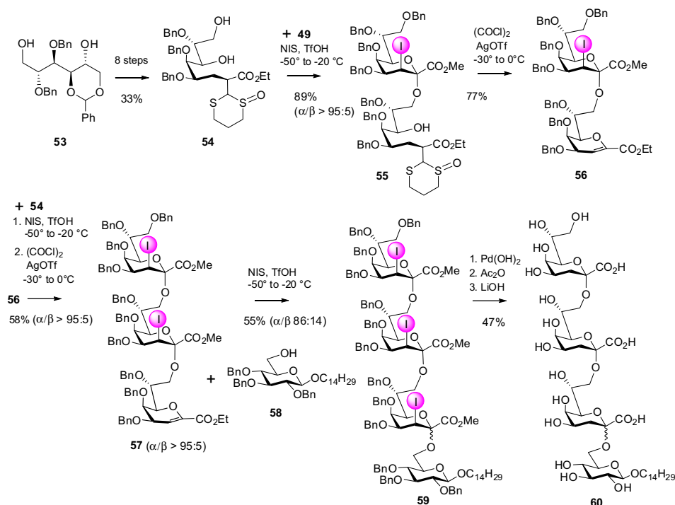
Scheme 11. Synthesis of \alpha -(2 \rightarrow 8)-Kdo trimers.
