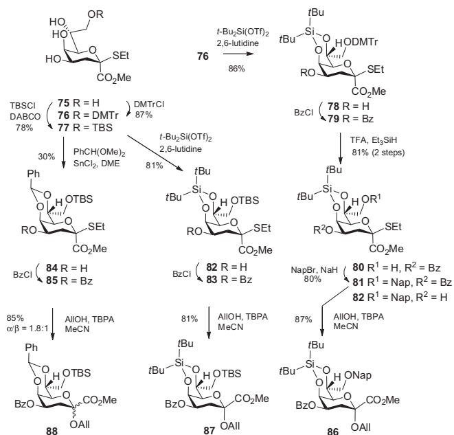
Scheme 15. Synthesis of 5,7-O-locked Kdo thioglycoside donor and acceptor derivatives.
