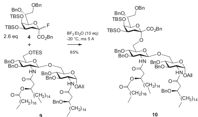
Scheme 2. Glycosylation of a 6-O-TES-protected diglucosamine acceptor.
