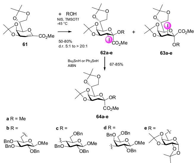
Scheme 12. Synthesis of \beta -Kdo derivatives.
