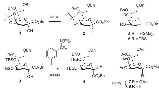
Scheme 1. Synthesis of Kdo fluoride donors.
