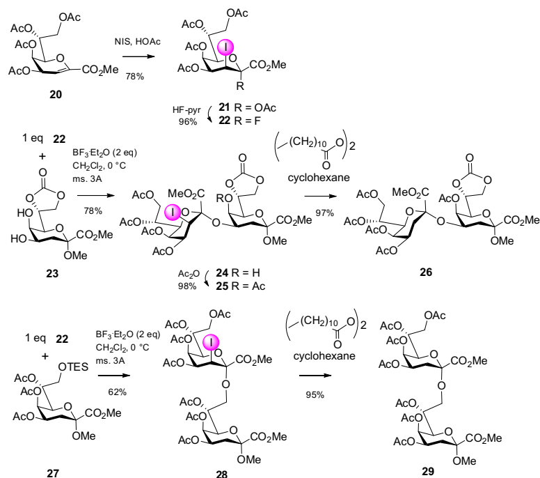
Scheme 5. Synthesis of Kdo disaccharides.
