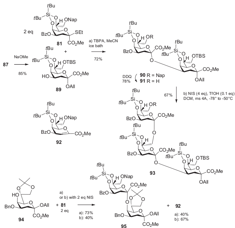
Scheme 16. Synthesis of the Chlamydia-related Kdo trisaccharide and the \alpha -(2 \rightarrow 5)-linked Kdo disaccharide.
