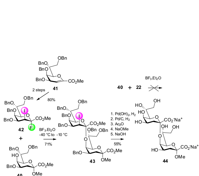
Scheme 8. Synthesis of the \alpha -(2 \rightarrow 5)-linked Kdo disaccharide 44.
