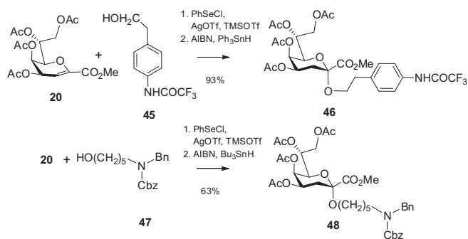
Scheme 9. Synthesis of spacer α-glycosides from glycal ester 20 .
