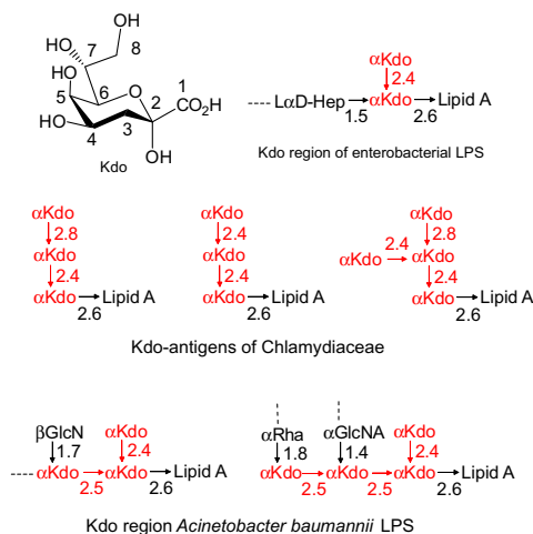
Figure 1. Numbering scheme for Kdo and structures of selected Kdo oligosaccharides from pathogenic bacteria.
