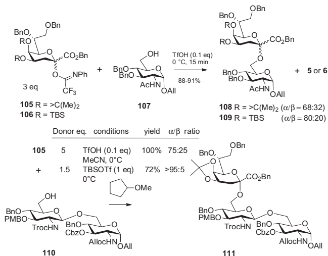
Scheme 18. Glycosylation reactions with Kdo N -phenyl trifluoroacetimidates.
