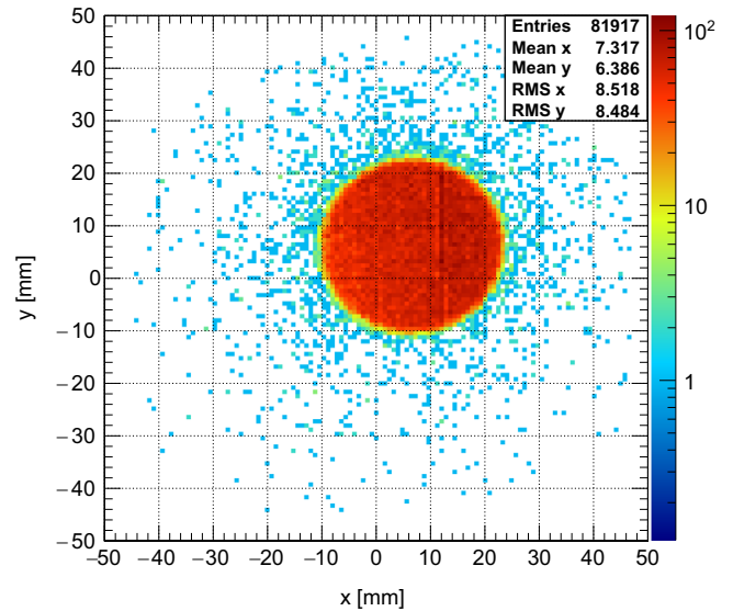
Fig. 8. The 2D reconstructed hit map of a 30 mm, 60 MeV proton beam at the Clatterbridge Cancer Centre. The distribution was reconstructed into 800 \mu\text{m} bins using two planes of the tracker unit orientated at 60° to one another.
