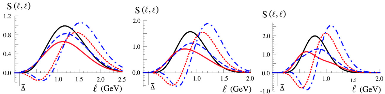
Fig. 2. Soft function S(\ell^+, \ell^-) as a function of \ell = \ell^+ = \ell^- with \mu = 1 GeV, at tree level (solid black line), one-loop (dotted red line), one-loop with renormalon subtraction (light solid red line), two-loop NLL (dot-dashed blue line), and two-loop NLL with renormalon subtraction (dashed blue line). Results are shown for three models: (a, b) = (2.5, -0.8) (left panel), (3.0, -0.5) (middle panel) and (3.5, -0.2) (right panel). All models have \Lambda = 0.55 GeV and a gap of \bar{\Delta} = 100 MeV. (For interpretation of the references to colour in this figure legend, the reader is referred to the web version of this Letter.)
