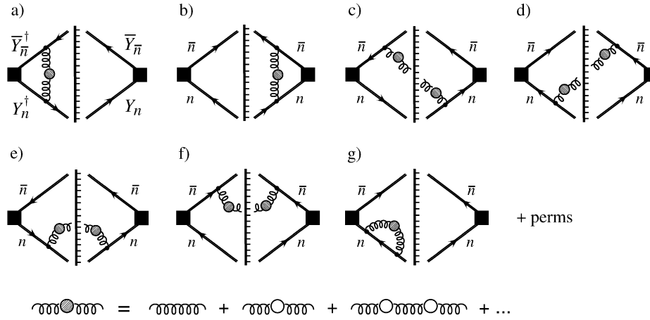
Fig. 1. Graphs for the hemisphere soft function with bubble chains. The solid lines denote Y -Wilson lines, and the line with ticks is the final state cut which may also cut a quark bubble.
