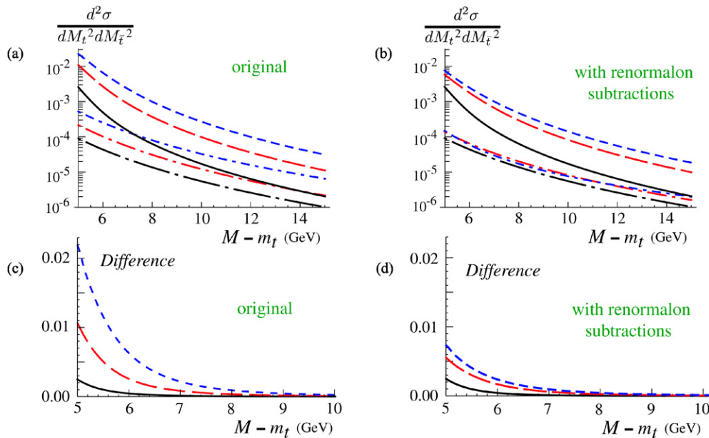
Fig. 5. Top invariant mass distribution d\sigma/dM_t^2 dM_{\bar{t}}^2 in the tail region as a function of M - m_t , with M = M_t = M_{\bar{t}} , \mu = (M^2 - m_t^2)/Q , and \bar{\Delta} = 100 MeV. In (a) results are shown without renormalon subtraction ( \delta = 0 ), and in (b) with a renormalon free gap parameter \bar{\Delta} . In (a), (b) we show: three curves using S_{\text{part}} at tree, 1-loop, \mathcal{O}(\alpha_s^2) NLL (long dot-dashed black, medium dot-dashed red, short dot-dashed blue), and three curves using the full S at tree, 1-loop, \mathcal{O}(\alpha_s^2) NLL (solid black, long dashed red, short dashed blue). The latter three curves use the model with \Lambda = 0.55 GeV and (a, b) = (3.0, -0.5) , and reflect the effects from power corrections when compared to the former three. In (c) and (d) we show the difference between the first and second set of three curves from (a) and (b) respectively, at tree (solid black), one-loop (long-dashed red), and \mathcal{O}(\alpha_s^2) NLL (short-dashed blue). (For interpretation of the references to colour in this figure legend, the reader is referred to the web version of this Letter.)
