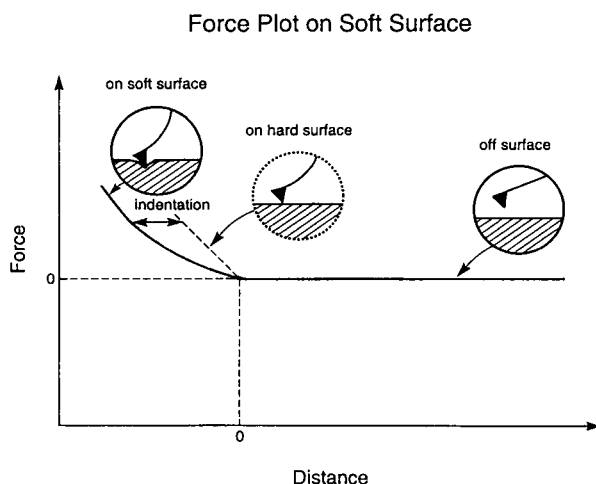
FIGURE 4 Diagrams of AFM force plots on A, hard and B, soft sample surfaces.
