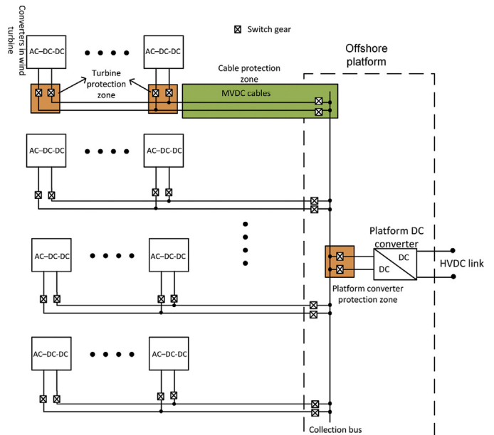
Fig. 7. Protection zones in DC collection systems.
