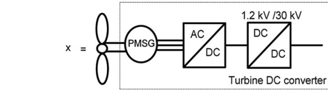
Fig. 2. DC1 collection systems.
