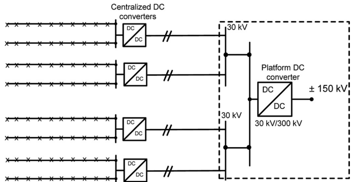
Fig. 2. DC1 collection systems.
