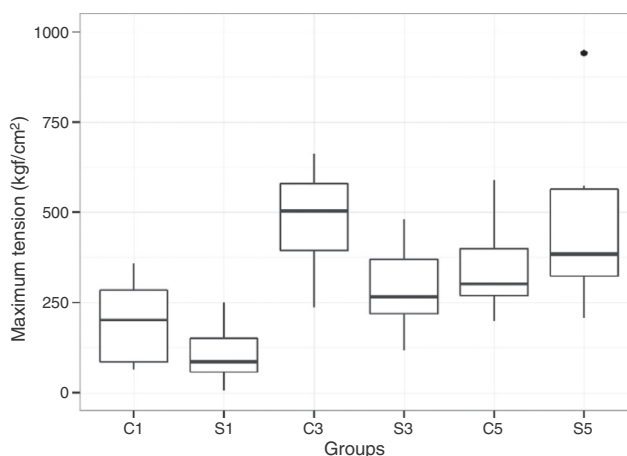
Fig. 4 – Boxplot showing distribution of the maximum tension among the groups.
