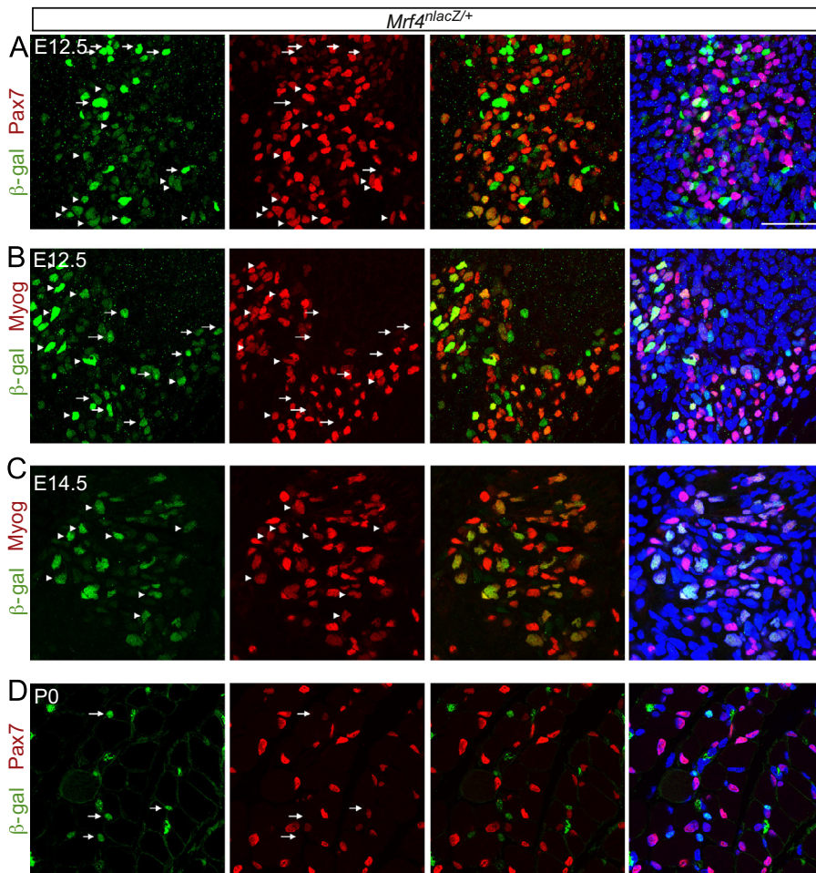
Fig. 6. Mrf4 induction in progenitors is restricted to the embryonic myogenic phase. (A–D) Immunostaining with anti- \beta -gal and anti-Pax7 (A, D) or Myog (B, C) antibodies on Mrf4^{lacZ} sections from embryonic (E12.5), foetal (E14.5) and post-natal (P0) phases. Sections for the top panels (A–C) were obtained from trunk at forelimb level, the P0 panels show a hindlimb section. Arrowheads point to double positive nuclei; arrows mark \beta -gal only expressing nuclei. Scale bar = 25 \mu .
