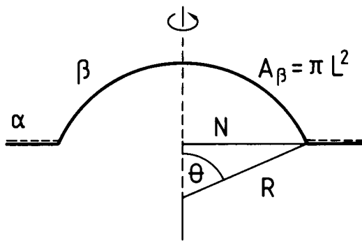
FIGURE 2 Bud geometry for the simple model in which the \beta domain of area A_\beta = \pi L^2 forms a spherical cap with curvature C . This cap is connected along its neck with radius N to the flat \alpha matrix.
