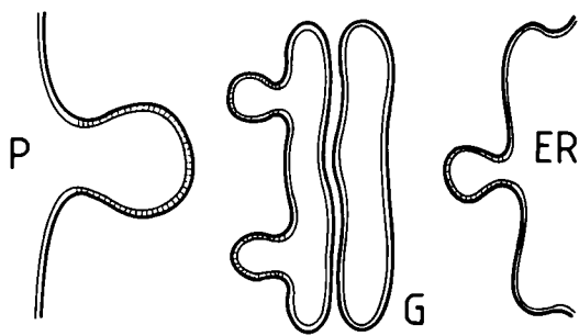
FIGURE 1 Highly schematic view of budding from the plasma membrane ( P ), from the Golgi apparatus ( G ), and from the endoplasmic reticulum ( ER ) of the cell.
