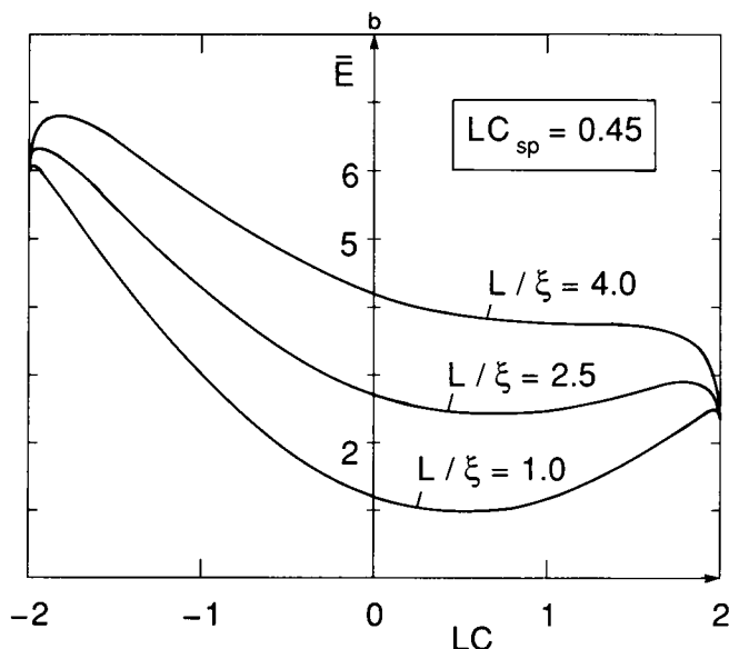
FIGURE 3 Reduced energy \bar{E} of the budding domain as a function of the reduced curvature LC : (a) for zero spontaneous curvature, C_{\text{sp}} = 0 , and (b) for nonzero spontaneous curvature with LC_{\text{sp}} = 0.45 . The length scale L denotes the linear size of the domain; the invagination length \xi = \kappa/\sigma , where \kappa and \sigma are the bending rigidity and the line tension of the domain edge. The uppermost curve corresponds to the size L = L^0 at which the incomplete bud becomes unstable.
