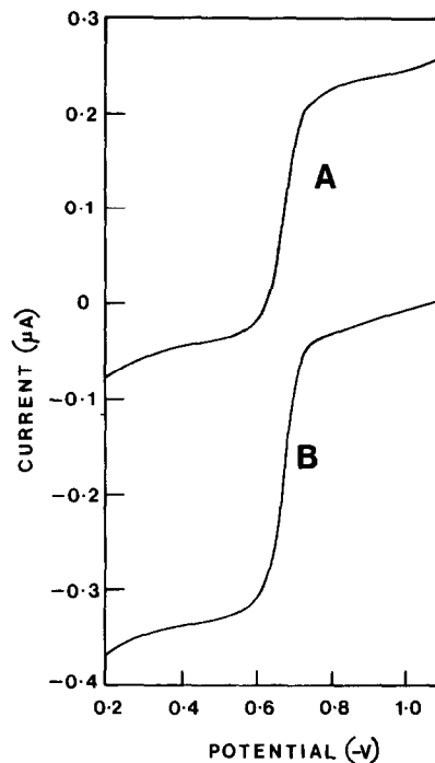
Fig. 3. Polarographic waves of oxidised and electroreduced lipoamide. Measurements were made on 40\ \mu\text{M} lipoamide in 0.1 M Tris-HCl, pH 8.0. A, oxidised lipoamide; B, dihydro-lipoamide. Current compensation of 0.25\ \mu\text{A}/\text{V} was applied.
