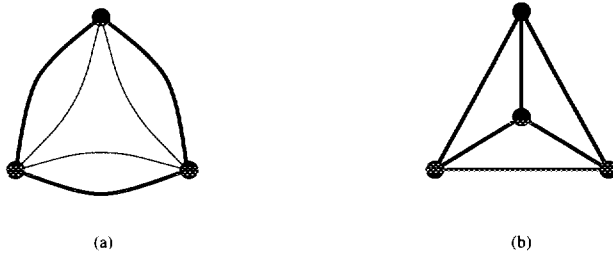
FIG. 2. Bold edges are in \Sigma .
