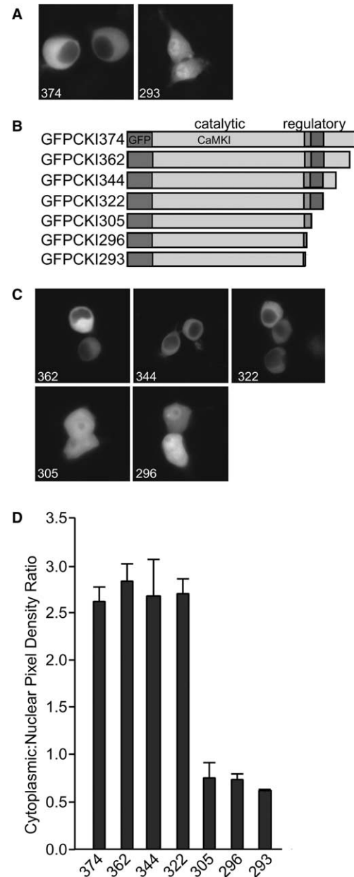
Fig. 1. Subcellular distribution of CaMKI- \alpha . (A) Fluorescence images of cells expressing GFP-CaMKI374 (374) and GFP-CaMKI293 (293). (B) Schematic representation of C-terminal truncations of CaMKI- \alpha . (C) Fluorescence images of cells expressing GFP-CaMKI362 (362), GFP-CaMKI344 (344), GFP-CaMKI322 (322), GFP-CaMKI305 (305), and GFP-CaMKI296 (296). (D) Cytoplasmic:nuclear ratios of GFP fluorescence in transfected cells. Error bars: \pm S.D. ANOVA: F(6, 115) = 69.59 . Post hoc tests revealed that C:N ratios of 374, 362, 344 and 322 were significantly different from those of 305, 296, 293 ( P < 0.001 ).
