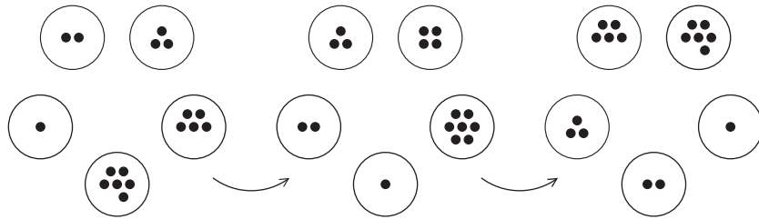
Fig. 1. A period of length 2; the active pit is drawn in bold.
