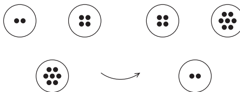
Fig. 4. Marching group M_{2,1} in an owari with 3 pits.
