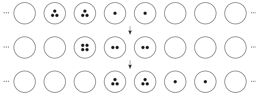
Fig. 3. Marching group of order 3, augmented by two pebbles.
