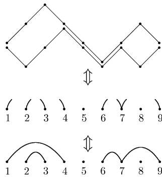
Fig. 2.3. A pair of noncrossing free Dyck paths and the corresponding partition.
