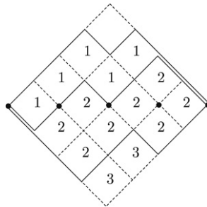
Fig. 2.1. A triple of noncrossing free Dyck paths and the corresponding plane partition.
