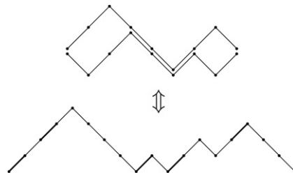
Fig. 3.1. The Labelle merging algorithm.
