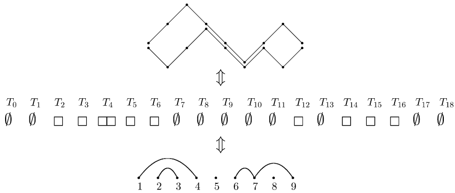
Fig. 2.2. A pair of noncrossing free Dyck paths and its corresponding partition.
