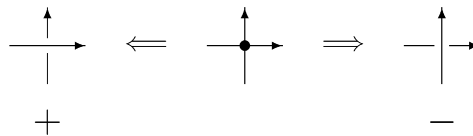
Fig. 3. Possible resolutions of a transverse self-intersection.
