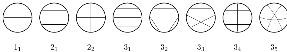
Fig. 1. Examples of chord diagrams.
