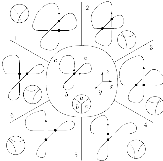
Fig. 2. Resolutions of a triple point.
