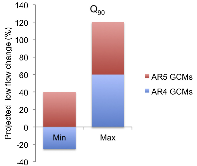
Fig. 5. Range of extreme streamflows projection for the 2050s based on results from two studies (Kim et al., 2008; Aich et al., 2014) for the upper Blue Nile basin using the previous (AR4) and new generation (AR5) of climate models.
