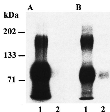
Fig. 1. Cross-linking of ^{125}\text{I} -rhTPO to human PB-derived megakaryocytes (A) and platelets (B). PB-derived megakaryocytes and washed platelets were exposed to the cross-linker \text{BS}^3 after incubation with ^{125}\text{I} -rhTPO in the absence (lane 1) or presence (lane 2) of a 200-fold excess of unlabeled rhTPO. Cell lysates were analyzed by SDS-polyacrylamide gel electrophoresis and autoradiography. The upper band represents the cross-linked complex and the lower band is free ^{125}\text{I} -rhTPO. The positions of molecular size markers are indicated in kilodaltons.
