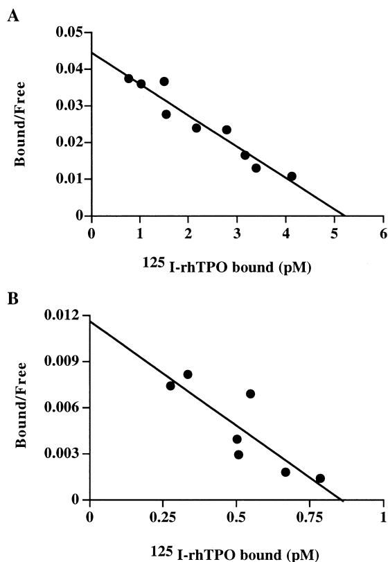
Fig. 2. Scatchard analysis of ^{125}\text{I-rhTPO} binding to CB-derived (A) and PB-derived (B) megakaryocytes. Cells were incubated with various concentrations of ^{125}\text{I-rhTPO} in the absence or presence of a 100-fold or more excess of unlabeled rhTPO for 1 h at 37°C. Data represent Scatchard analysis of representative experiments.
