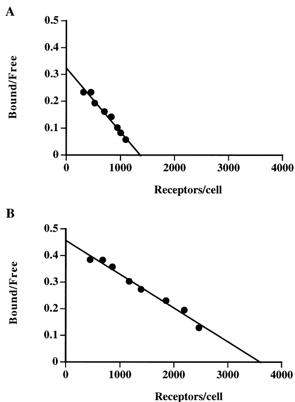
Fig. 3. Scatchard analysis of ^{125}\text{I-rhTPO} binding to Dami cells cultured in the absence (A) or presence (B) of TPA. Cells were cultured for 20 days in the absence or presence of 5 nM TPA, after which the binding of ^{125}\text{I-rhTPO} was assessed by Scatchard analysis. Data are from a representative experiment and revealed 1351 (A) and 3508 (B) receptors per cell.
