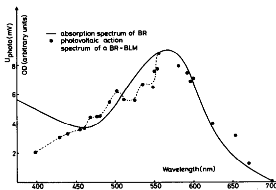
Fig.3. Open-circuit photovoltaic action spectrum of a bimolecular lipid membrane containing bacteriorhodopsin. The action spectrum has been corrected to correspond to equal quantum numbers of incident monochromatic light. Excitation intensity was 10^{13} \text{ quanta cm}^{-2} \text{ s}^{-1} at any wavelength. The absorption spectrum of the purple membrane in aqueous dispersion is indicated by the full line.
