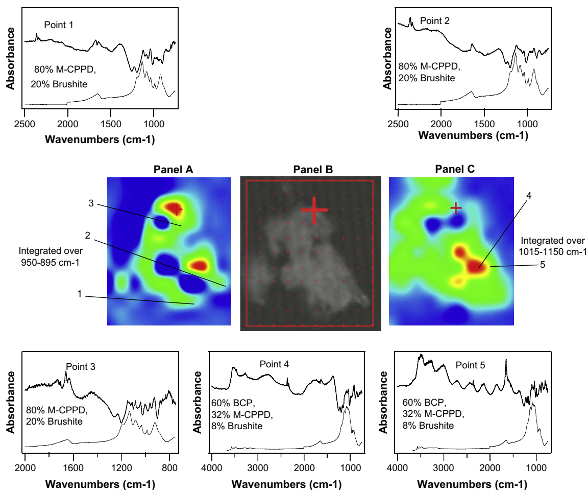
Fig. 6. sFTIR map of a typical crystal generated by ACVs. The data, 110 pixels over the entire area were collected with 12 \times 12\text{-}\mu\text{m}^2 aperture and 64 scans per pixel. Panel B shows a visible image of the crystal with red dots showing the location of each pixel of data. Infrared images (panels A and C) are shown that are dominated by the absorbance of functional groups specific to BCP (panel A) and CPPD (panel C). The spectral range for BCP was 985\text{--}895\text{ cm}^{-1} and for CPPD was 1015\text{--}1150\text{ cm}^{-1} . Red areas on the infrared images indicate high absorption intensity and can be indicative of the presence of the crystal functional group, whereas blue areas indicate low absorption intensity by functional group and absence of the functional group. The remaining panels (points 1–5) show standard spectra and data in a given pixel for the pixels identified in the infrared images and compare them to combinations of CPPD, BCP and brushite. All of the sample spectra contain additional peaks arising from admixture of biologic material. The infrared images and spectra suggest superimposed areas of CPPD, BCP and brushite minerals in a single crystal aggregate.
