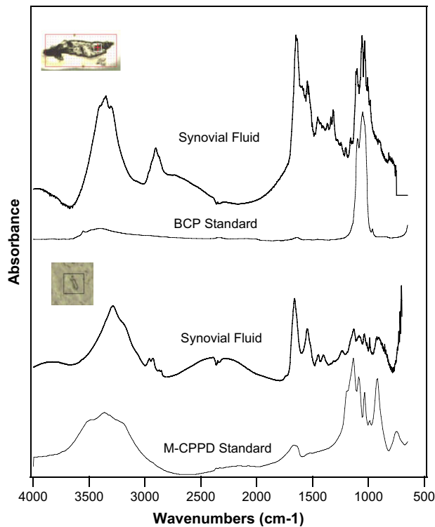
Fig. 1. Representative sFTIR spectra from human synovial fluids demonstrating CPPD and BCP crystals. The crosshairs in the visible images indicate the points at which the measurements were obtained. The top sample spectrum was collected with a 10 \times 10\text{-}\mu\text{m}^2 aperture and 64 scans, while the bottom sample spectrum was collected with an 8 \times 8\text{-}\mu\text{m}^2 aperture and 64 scans. For the latter crystal, the sample is clearly smaller than the 8 \times 8\text{-}\mu\text{m}^2 aperture, but is completely within the field of view. The infrared signatures produced by the synovial fluid crystals clearly match the standard spectra of BCP and CPPD crystals, respectively. The additional peaks on the synovial fluid crystal spectra suggest the presence of biologic material mixed with the crystals.
