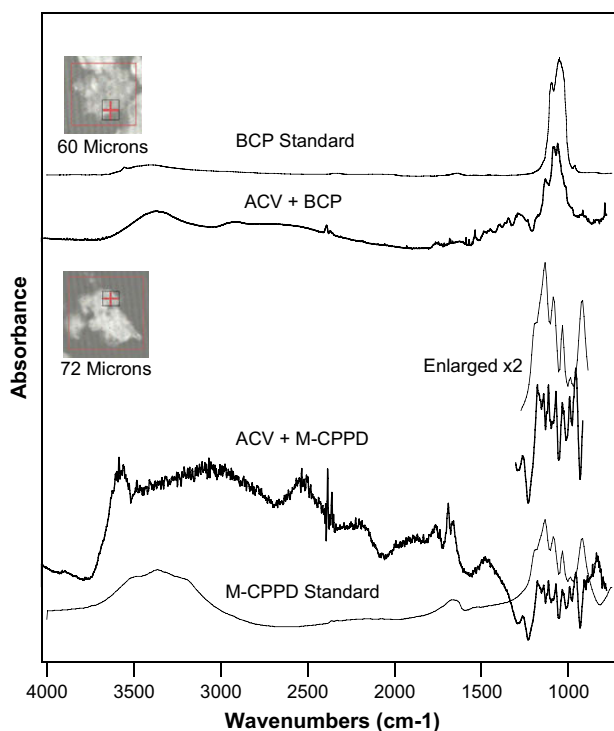
Fig. 3. Representative sFTIR spectra from porcine ACVs. ACVs were incubated for 3–5 days with either 1-mM ATP or 1-mM \beta -glycerophosphate. The crosshair identifies the point at which the image was collected for each sample. The top sample spectrum was collected with a 15 \times 15 - \mu\text{m}^2 aperture as shown and 64 scans, while the bottom sample spectrum was collected with a 12 \times 12 - \mu\text{m}^2 aperture as shown and 64 scans. The data for the mCPPD standard and the ACV-generated CPPD-like crystal have been multiplied by two and offset below 1500 cm -1 to emphasize the comparison between the spectra. The spectrum for the top sample is similar to BCP and that the spectrum for the bottom sample is similar to mCPPD.
