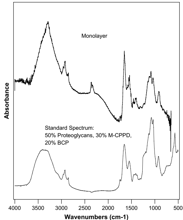
Fig. 5. Representative sFTIR spectrum from a crystal generated by chondrocyte monolayers and a mixture of BCP, CPPD and proteoglycans. The sFTIR spectrum from a crystal generated by chondrocyte monolayers was compared with an FTIR spectrum generated by a combination of 50% cartilage proteoglycans, 30% mCPPD, and 20% BCP.
