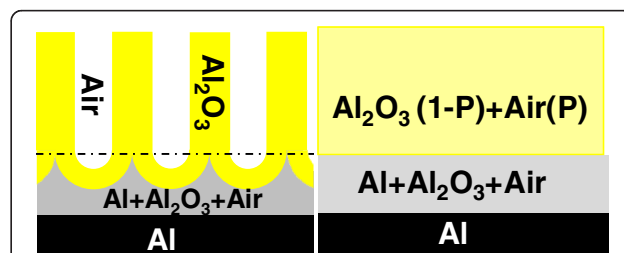
Figure 1 Sketch of the structure used to model the ellipsometric data. Left: schematic drawing of the NAA structure showing the pores, the alumina, and the aluminum substrate. Right: the corresponding layered optical model considered by the characterization software. P is the porosity of the NAA, which corresponds to the volume fraction of air. The plus sign represents the use of a Bruggeman effective medium approximation to model the refractive index of the mixture of materials in the layer.
