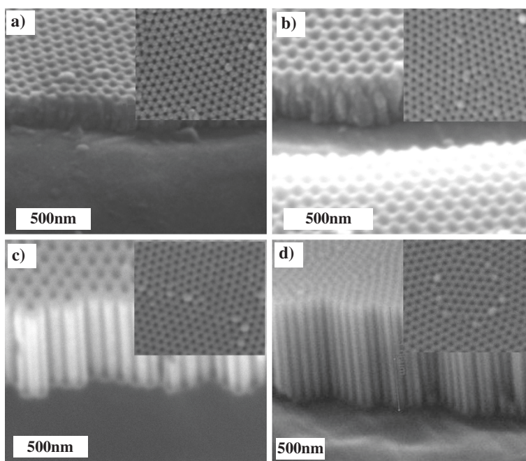
Figure 3 Set of ESEM images of the as-anodized NAA fabricated with different applied voltages. (a) 20, (b) 30, (c) 40, and (d) 50 V. All the samples were obtained after 10 min of anodization.
