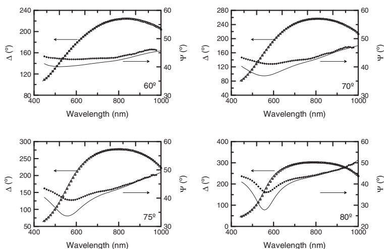
Figure 2 Ellipsometric measurements for the sample 110928-A11 (symbols). Together with the best fit (considering all the angles of incidence simultaneously) obtained with the DeltaPsi2 software. The corresponding measurement angle of incidence is indicated in each graph.
