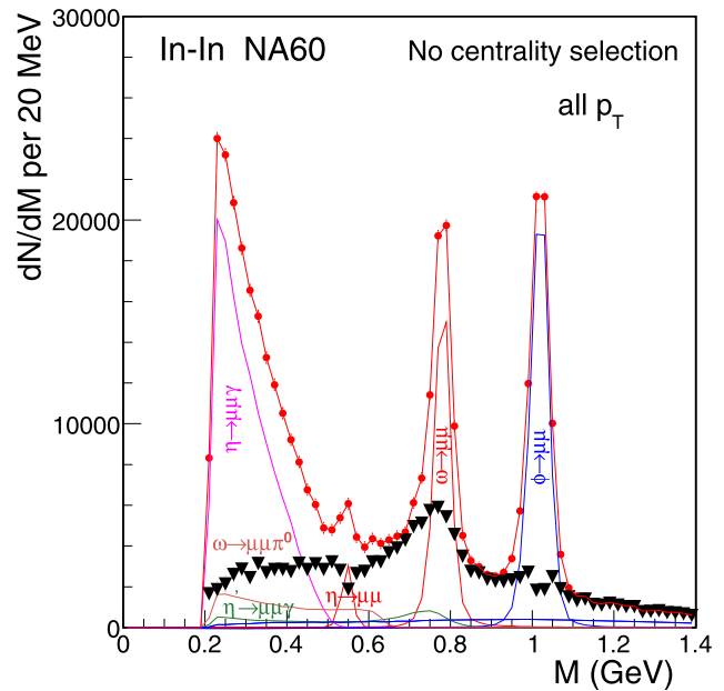
Fig. 2.1 Background-subtracted mass spectrum before ( dots ) and after subtraction of the known decay sources ( triangles )
