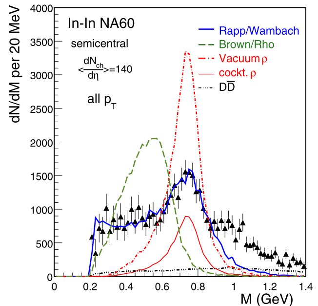
Fig. 2.2 Excess dimuons compared to theoretical predictions [16], renormalized to the data in the mass interval M < 0.9 GeV. No acceptance correction applied
