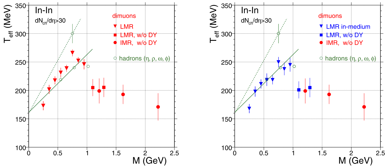
Fig. 4.5 Left: Inverse slope parameter T_{\text{eff}} vs. dimuon mass for the combined LMR/IMR regions of the excess in comparison to hadrons [13]. Right: Inverse slope parameters T_{\text{eff}} for the “pure” in-medium part, obtained by subtraction of the \rho -peak contribution from
