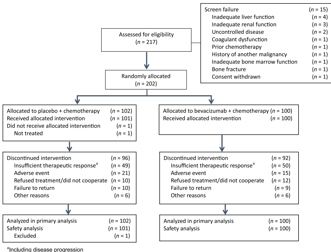
Fig. 1 CONSORT diagram
