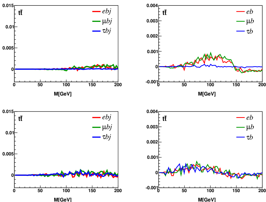
Figure 13. Invariant mass distributions for t\bar{t} events. The left panels show \ell b_{\text{jet},j} distributions and the right panels show \ell b_{\text{jet}} distributions. In the upper panels the loose cut is used and in the lower panels the pT_{\text{miss}} cut is used and R_{\text{jet}} = 0.2 .
