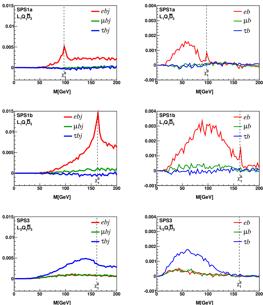
Figure 10. Left panels: \ell b_{\text{jet}} j distributions with same-sign subtraction in the \ell b_{\text{jet}} pair. Right panels: \ell b_{\text{jet}} distributions with same-sign subtraction. Upper and middle panels: L_1 Q_1 \bar{D}_3 at SPS1a (upper) using the loose cut and SPS1b (middle) using the hard cut. Lower panels: L_3 Q_1 \bar{D}_3 at SPS3 with R_{\text{jet}} = 0.2 and using the pTmiss cut.
