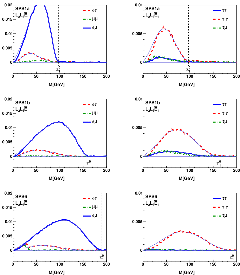
Figure 5. Comparison between fitted theoretical distributions (thin curves in violet) and Monte Carlo results (heavy curves). The results for L_2L_3\bar{E}_1 are shown for three different SPS points.
