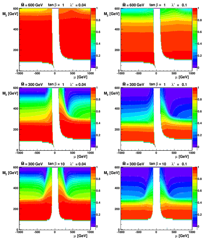
Figure 2. Dominance of MSSM decay of squark vs its R-parity-violating decay, shown for two squark masses, and two values each of \tan\beta and \lambda' .
