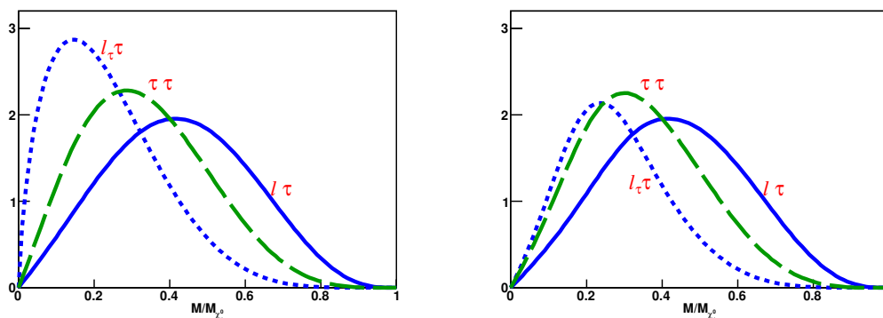
Figure 21. Effects of cuts on invariant mass distributions involving taus. Left: No cuts. Right: Cuts as indicated by eq. (B.11). Long-dashed (green) curve: two tau jets are combined; solid (blue): one directly produced lepton combined with a tau jet; short-dashed (blue): a tau together with a lepton from a tau decay.
