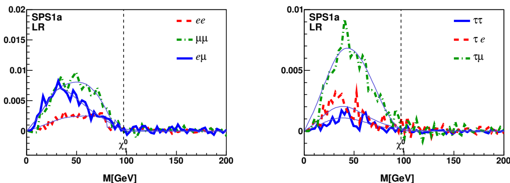
Figure 16. The same as figure 5 for the Left-Right symmetric scenario defined by (6.4) at SPS1a.
