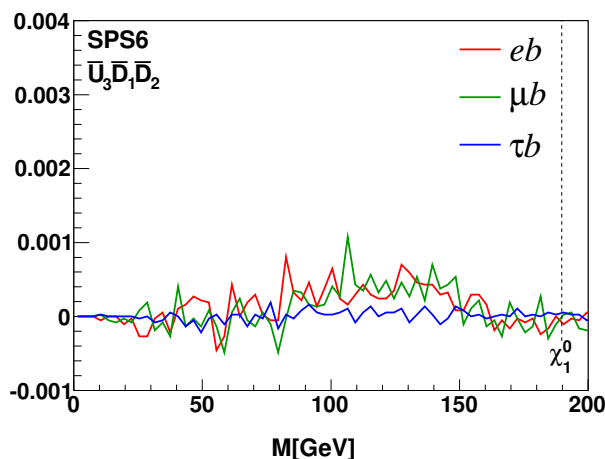
Figure 14. Invariant mass distributions for \chi''_{312} at SPS6. The distributions shown are lb_{\text{jet}} distributions for all lepton flavours.
