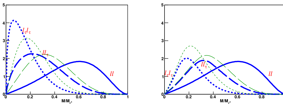
Figure 20. Theoretical invariant di-lepton mass distributions for massless particles from \tilde{\chi}_1^0 decay. Left: No cuts. The \ell\ell curve is given by eq. (B.2). Right: Cuts as indicated by eq. (B.11). Solid curves: directly produced leptons; long-dashed curves: one lepton comes from a decaying tau; short-dashed curves: both leptons come from decaying taus. Blue heavy curves do not take tau polarization into account while the thin green curves do. The labels refer to the heavy curves (blue).
