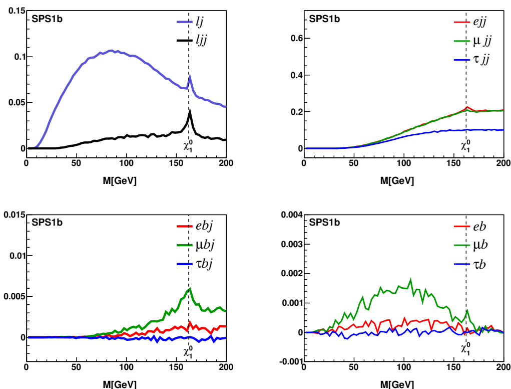
Figure 11. Combinations of LQ\bar{D} operators: Invariant masses for \lambda'_{121} = 10^{-4} and \lambda'_{223} = 10^{-4} at SPS1b. The two operators differ both in lepton flavours and in quark flavours. Upper left: l_j and l_{jj} (magnified by a factor 5), in the latter case the two jets are close to the lepton (see figure 9). Upper right: l_{jj} . Lower panels show l_{b_{jet},j} (left) and l_{b_{jet}} (right) distributions. All plots use the hard cut.
