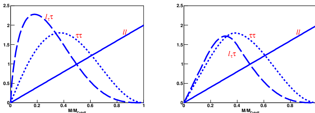
Figure 22. Invariant mass distributions expected from the higher RPC chain. Left: No cuts. Right: Cuts as indicated by eq. (B.11). Solid: the familiar triangular di-lepton distribution; short-dashed: the di-tau-jet invariant mass; long-dashed: lepton-tau-jet mass distribution, expected when one of the taus decays leptonically.
