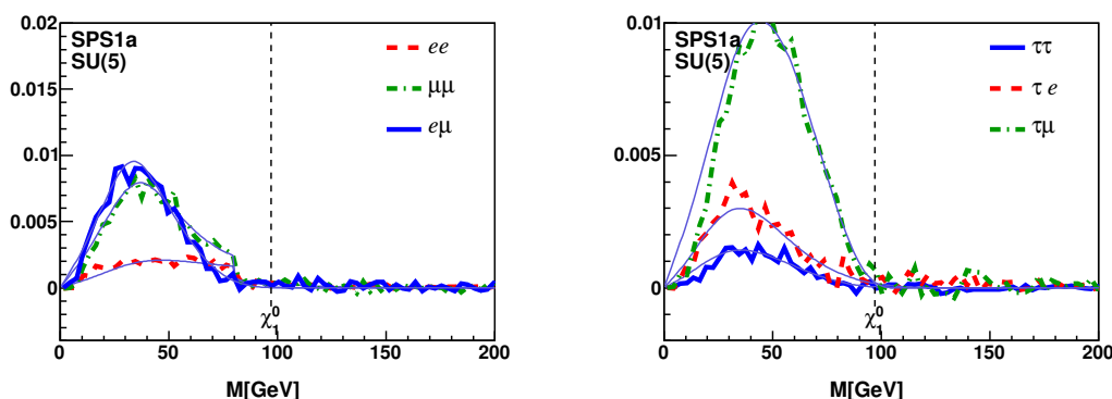
Figure 17. The same as figure 5 for the SU(5) scenario defined by tables 12 and 13 at SPS1a.
