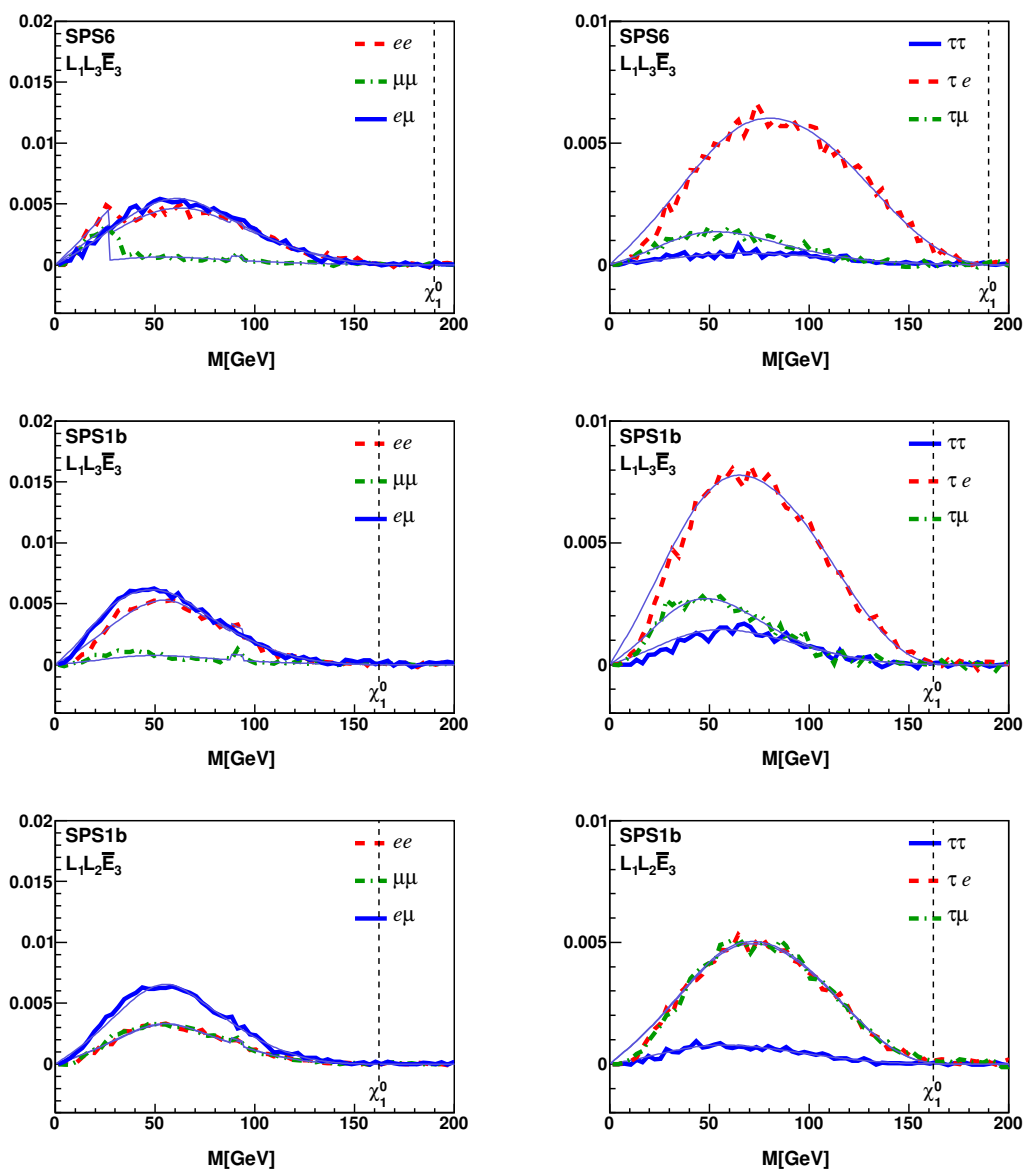
Figure 6. The same as figure 5 for some tau-rich operators at SPS1b and SPS6.
