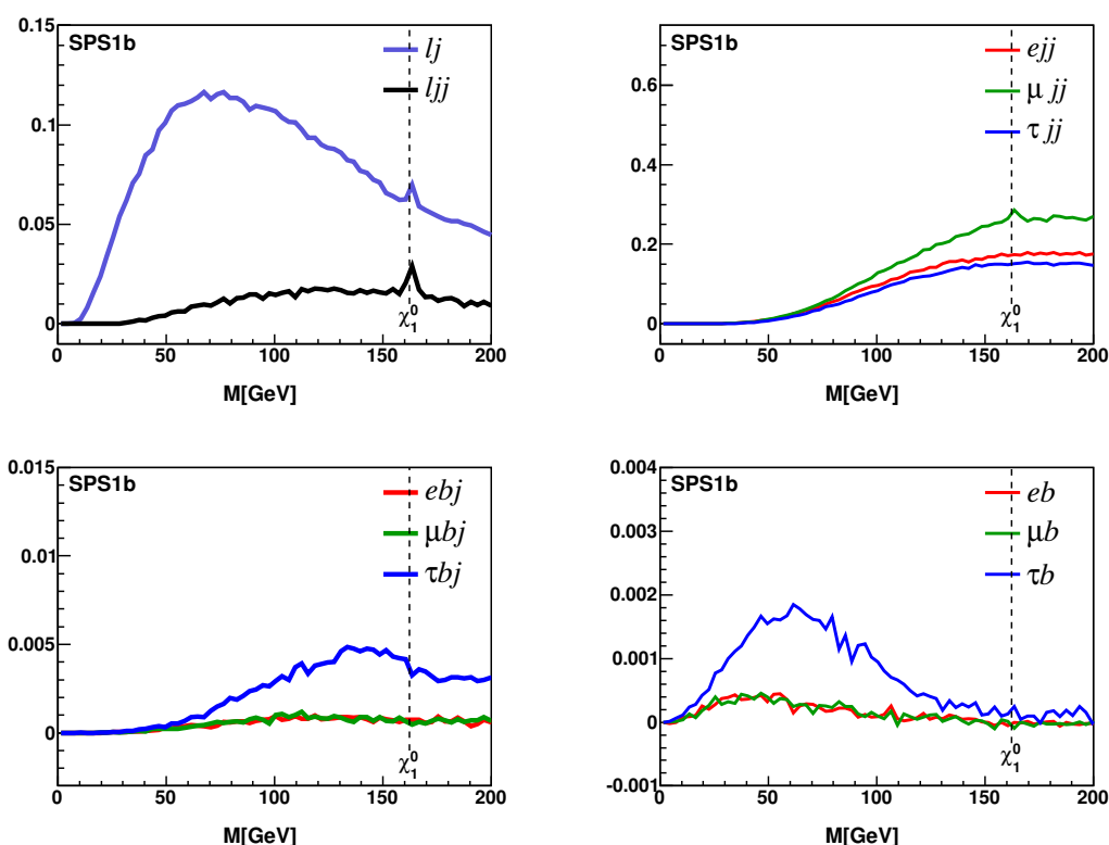
Figure 12. Same as figure 11 for \lambda'_{211} = 10^{-4} and \lambda'_{313} = 10^{-4} at SPS1b. Here the two lower panels use the pTmiss cut as well as R_{\text{jet}} = 0.2 to get enough \tau_{\text{jet}} 's.
