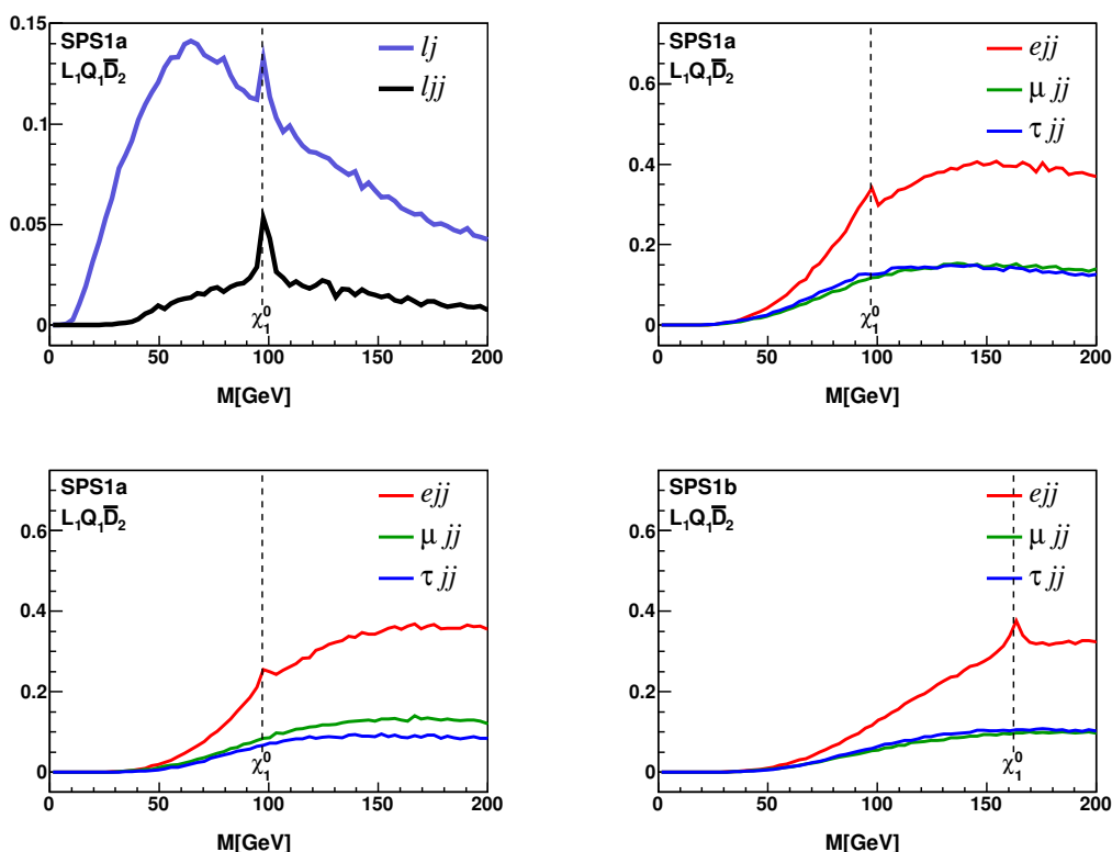
Figure 9. Invariant mass distribution for L_1Q_1\bar{D}_2 at SPS1a: upper left: violet: lj distribution, black: ljj where the jets are closer than \Delta R = 1 to the lepton, this distribution has been multiplied by 5 to be visible. Upper right: ljj distributions using R_{\text{jet}} = 0.2 . Lower left panel: same as upper right but with R_{\text{jet}} = 0.4 , lower right: same as lower left but for SPS1b. In this figure, the hard cut has been used.
