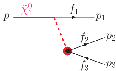
Figure 18. Kinematics of three-body neutralino decay.
