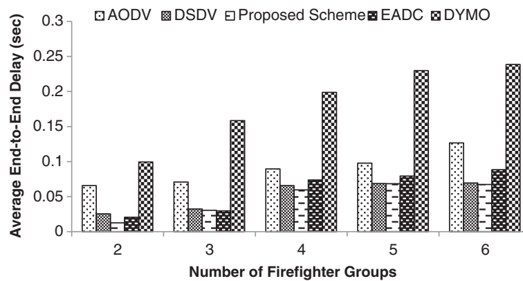
Figure 3 Average end-to-end delay for five schemes with an increasing number of firefighter groups.
