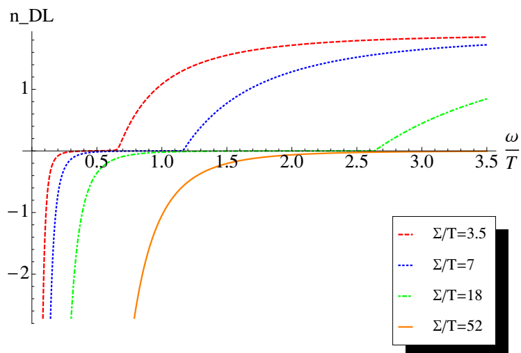
Figure 1. n_{DL} for different values of \Sigma/T and q = 0.05 .
