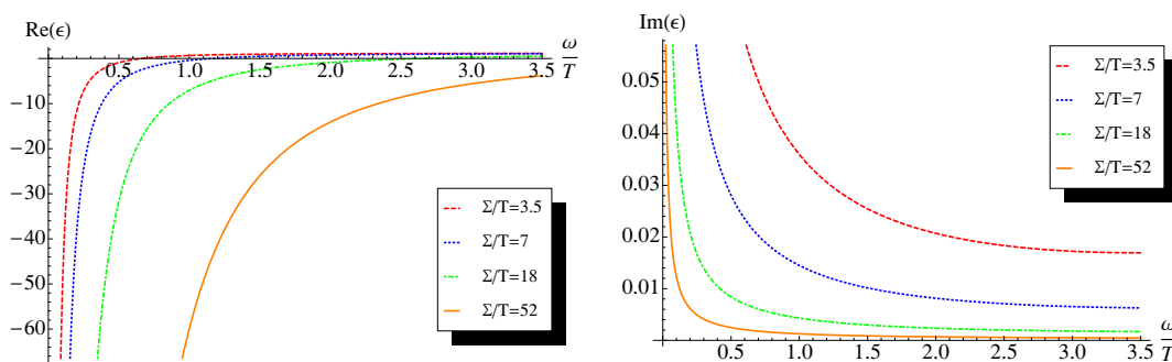
Figure 3. \text{Re}[\epsilon(\omega)] and \text{Im}[\epsilon(\omega)] for different values of \Sigma/T and q = 0.05 .
