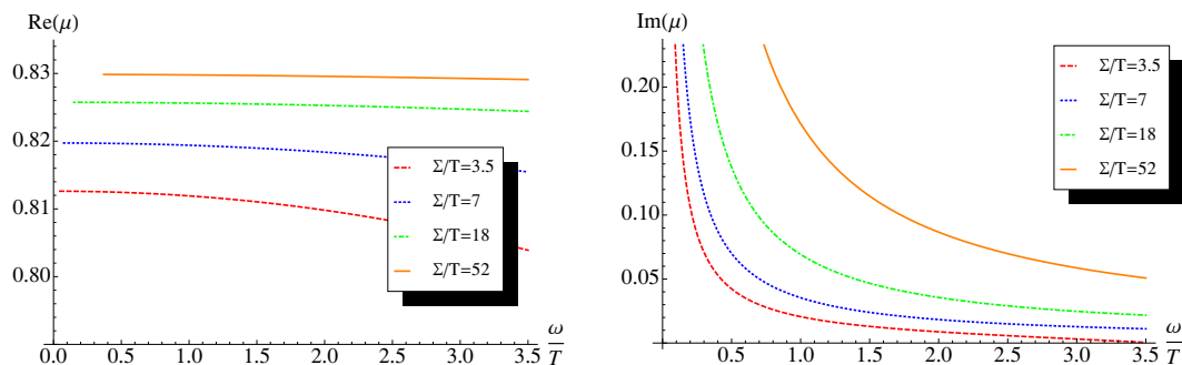
Figure 4. \text{Re}[\mu(\omega)] and \text{Im}[\mu(\omega)] for different values of \Sigma/T and q = 0.05 .
