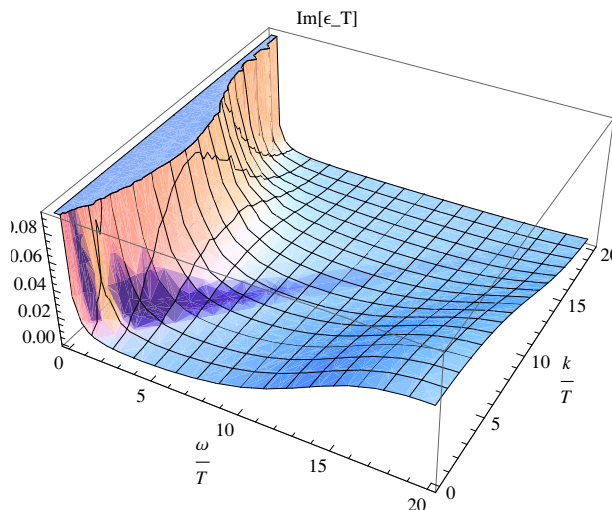
Figure 2. \text{Im}(\epsilon_T) as a function of \frac{\omega}{T} and \frac{k}{T} , with \Sigma/T = 7.5 and q = 0.05 .
