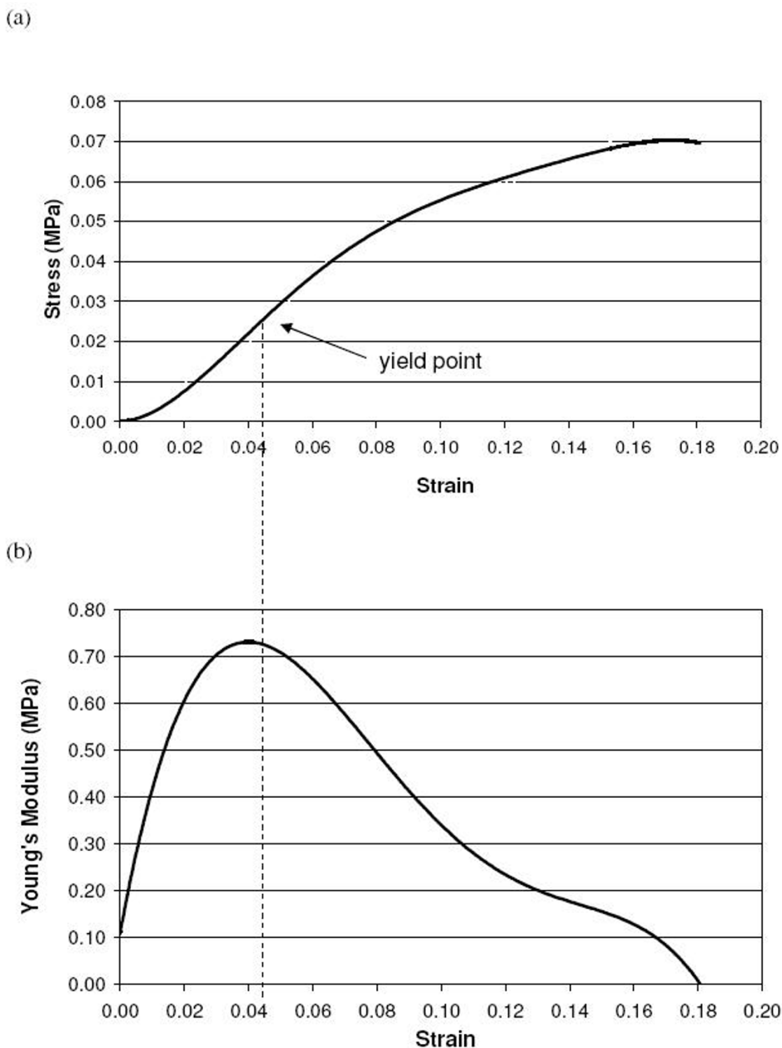
Figure 1 Stress-strain and Young's modulus-strain curves. (a) Stress-strain curve from a 7.7 mm length sample of open cell PU foam ( 0.09 \text{ g}\cdot\text{cm}^{-3} ) used to model very low density human cancellous bone and (b) the Young's modulus determined from it as the gradient of the curve. The yield point is defined by the point at which the Young's modulus decreases by 3% from its maximum value. The area under the stress-strain curve up to the yield point is defined as the energy absorbed to yield.
