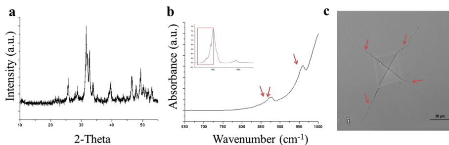
Figure 4 XRD, FTIR spectrums and SEM micrograph of Vicker's microindentation on tooth enamel samples. (a) XRD spectrum of tooth enamel powder, (b) FTIR absorbance spectra of tooth enamel samples normalized to absorbance peak of v_3PO_4 at 1013\text{ cm}^{-1} (arrows show the peaks that used for the calculation of carbonate content), (c) SEM micrograph of Vicker's microindentation on enamel (cracks are shown by arrows on the corners of indentation).
