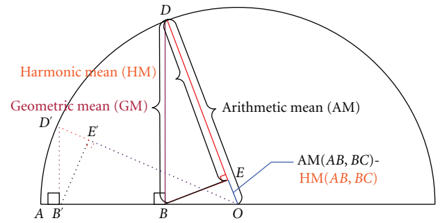
FIGURE 7: Geometrical interpretation of the harmonic mean, the arithmetic mean, and the geometric mean of AB(A'B') and BC(B'C') .
