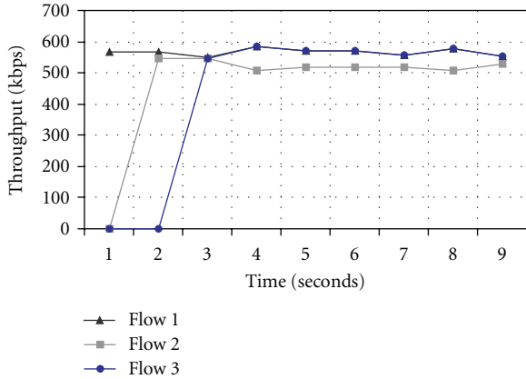
FIGURE 2: Throughput of three flows (1, 2, 3) versus time. RTS/CTS mechanism is enabled.
