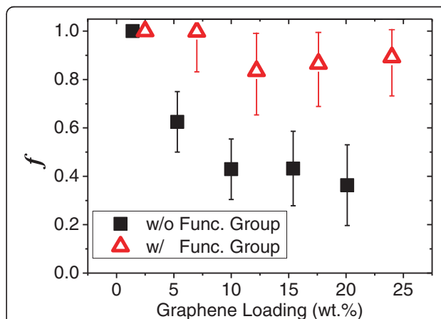
Fig. 6 The dispersion ratio f as a function of the graphene loading. Without functional groups, the degree of dispersion decreased with increasing graphene loading. With functional groups, however, the degree of dispersion was almost independent of the graphene loading
