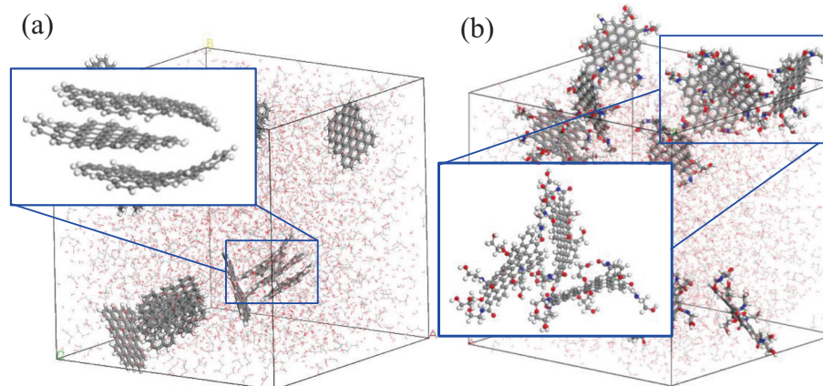
Fig. 4 Snapshots of molecular dynamics (MD) simulations for nanofluids containing a 10.0 wt.% graphene and b 12.4 wt.% functionalized graphene. The enlarged images show that a graphene sheets tended to stack to form aggregates, but that b the functionalized graphene did not stack
