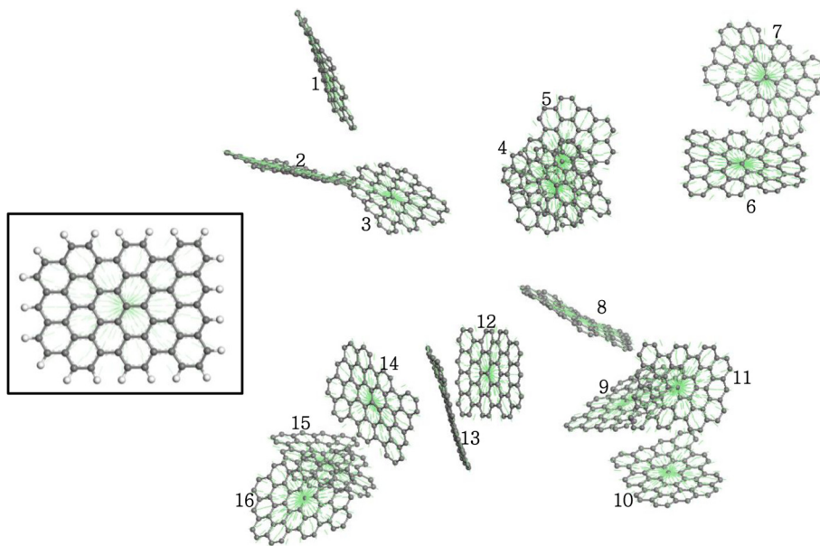
Fig. 2 The numbering of centroids of graphene sheets used to calculate the degree of dispersion in a nanofluid. The inset shows where the centroid occurs in the graphene sheets. If the separation between graphene sheets becomes smaller than 3.5 times the carbon-carbon Van der Waals separation, the graphene sheets are considered aggregated
