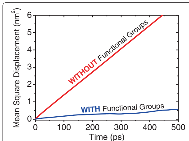
Fig. 5 Comparison of MSD between graphene sheet with and without functional groups, at 1.4 and 2.5 wt.%, respectively. The slope of MSD without functional groups is much steeper than that of with. We concluded that this result came from affinity of functional groups to surrounding fluids
