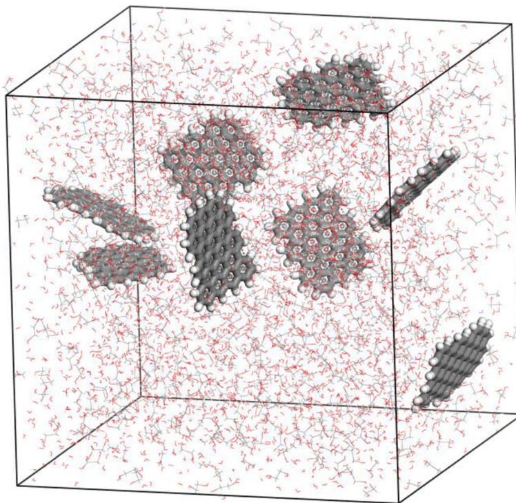
Fig. 1 A snapshot of a molecular dynamics simulation of a 5.3 wt.% dispersion of graphene in a 1:1 mixture of water and ethylene glycol (EG)
