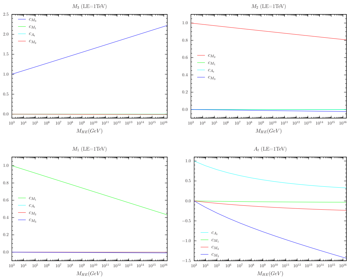
Figure 7. Left to right, top to bottom: as figure 3, for M_3(M_{LE}) , M_2(M_{LE}) , M_1(M_{LE}) and A_t(M_{LE}) .
