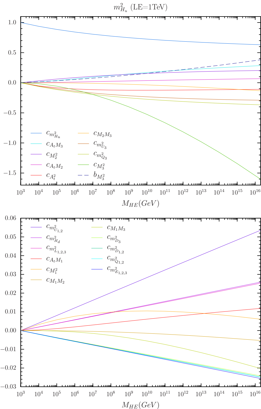
Figure 4. m_{H_u}^2(M_{LE}) coefficients dependence on the HE scale, for M_{LE} = 1 \text{ TeV} and \tan \beta = 10 . For further details, see eqs. (A.1)–(A.3).
