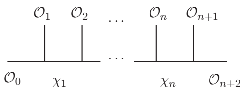
Figure 1. The comb diagram of an n -channel linear conformal block. The initial and final states, \mathcal{O}_0 and \mathcal{O}_{n+2} , the vertex operators \mathcal{O}_i , i = 1, \dots, n + 1 , and the \mathcal{W}_N irreducible highest weight representation that flows in the \iota -th channel \chi_\iota , \iota = 1, \dots, n , are defined in the text.
