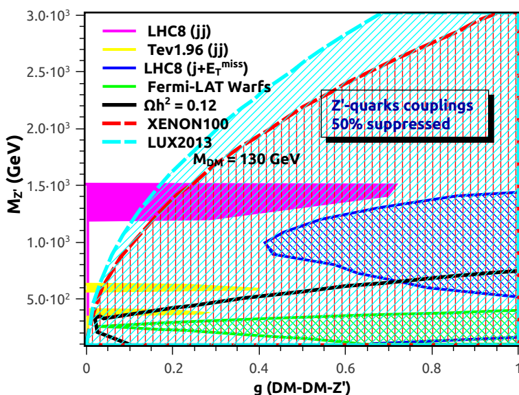
Figure 10. Result for M_\chi = 130 \text{ GeV} in the M_{Z'} \times \text{DM-DM-}Z' coupling plane, with Z' -quarks couplings suppressed. The white regions are not ruled out by any constraint. The pink region is ruled out by the LHC 8 TeV using the dijet data. Yellow is excluded by Tevatron (1.96 TeV) with the dijet data. The dashed blue region is excluded by LHC at 8 TeV using the jet + E_T^{\text{miss}} analysis. The red dashed region is the XENON100 excluded region. The black line reproduces \Omega h^2 = 0.12 , whereas the regions above and beneath the black curve set \Omega h^2 > 0.12 and \Omega h^2 < 0.12 respectively.
