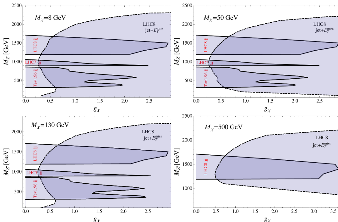
Figure 2. Exclusion regions from Tevatron, LHC 7 and 8 TeV searches for resonances in dijet events and from monojet search at the LHC 8 TeV in the M_{Z'} versus g_{\chi} plane. The left upper panel shows the 95% C.L. excluded region for a fixed DM mass of 8 GeV, while the upper right, the lower left, and lower right panels show the cases for a 50, 130, and 500 GeV, respectively. Additional collider bounds are presented further.
