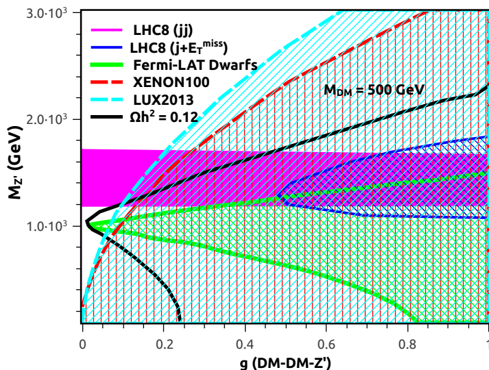
Figure 13. Result for M_{\chi} = 500 GeV in the M_{Z'} \times \text{DM-DM-}Z' coupling plane. The gaps evade all bounds. The pink region is ruled out using the dijet data from the LHC 8 TeV. The dashed blue region is excluded by LHC at 8 TeV using the jet + E_T^{\text{miss}} analysis. The red dashed region is the XENON100 excluded region. The black line reproduces \Omega h^2 = 0.12 , whereas the regions above and below the lines set \Omega h^2 > 0.12 and \Omega h^2 < 0.12 respectively.
