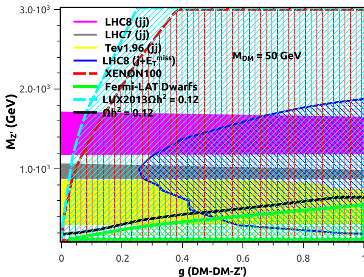
Figure 11. Result for M_\chi = 50 GeV in the M_{Z'} \times \text{DM-DM-}Z' coupling plane. The white regions are not ruled out by any constraint. Pink and Grey regions are ruled out by the LHC 8 TeV and 7 TeV using the dijet data. Yellow is excluded by Tevatron (1.96 TeV) with the dijet data. The dashed blue region is excluded by LHC at 8 TeV using the jet + E_T^{\text{miss}} analysis. The red dashed region is the XENON100 excluded region. The black line reproduces \Omega h^2 = 0.12 , whereas the regions above and below the lines set \Omega h^2 > 0.12 and \Omega h^2 < 0.12 respectively.
