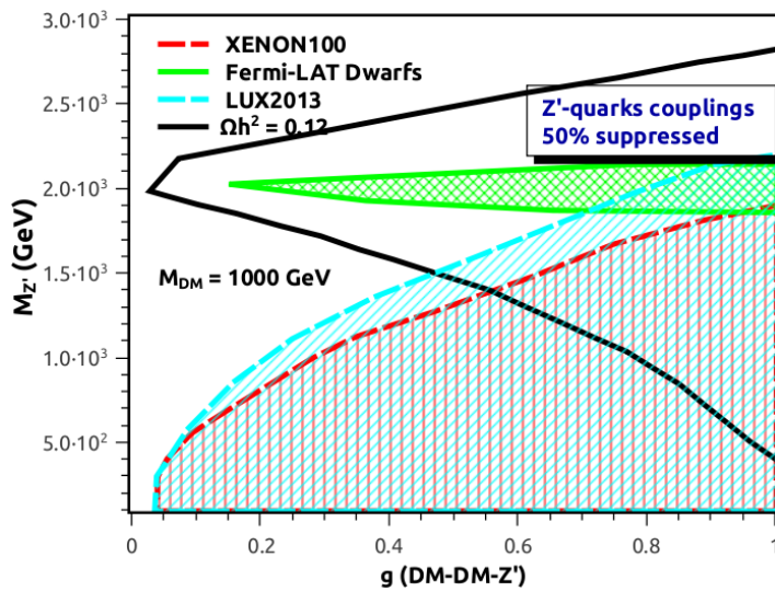
Figure 16. Result for M_{\chi} = 1000 GeV in the M_{Z'} \times DM-DM- Z' coupling plane, with Z' -quarks couplings suppressed. The white regions are not ruled out by any constraint. The red dashed region is the XENON100 excluded region. The black line reproduces \Omega h^2 = 0.12 , whereas the regions above and below the lines set \Omega h^2 > 0.12 and \Omega h^2 < 0.12 respectively.
